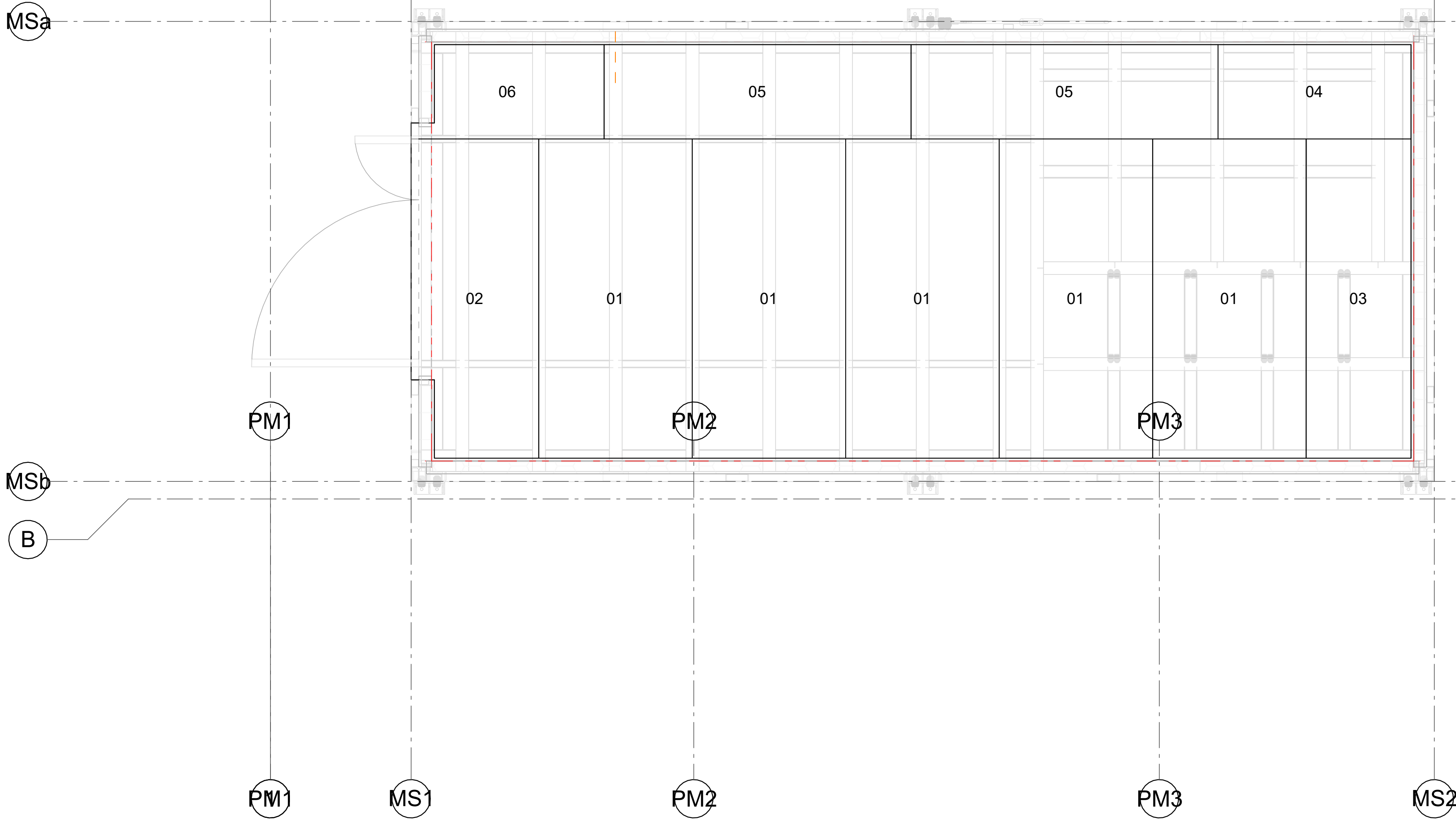
PM - FIRST FLOOR LAYER LAYOUT - PLYWOOD
