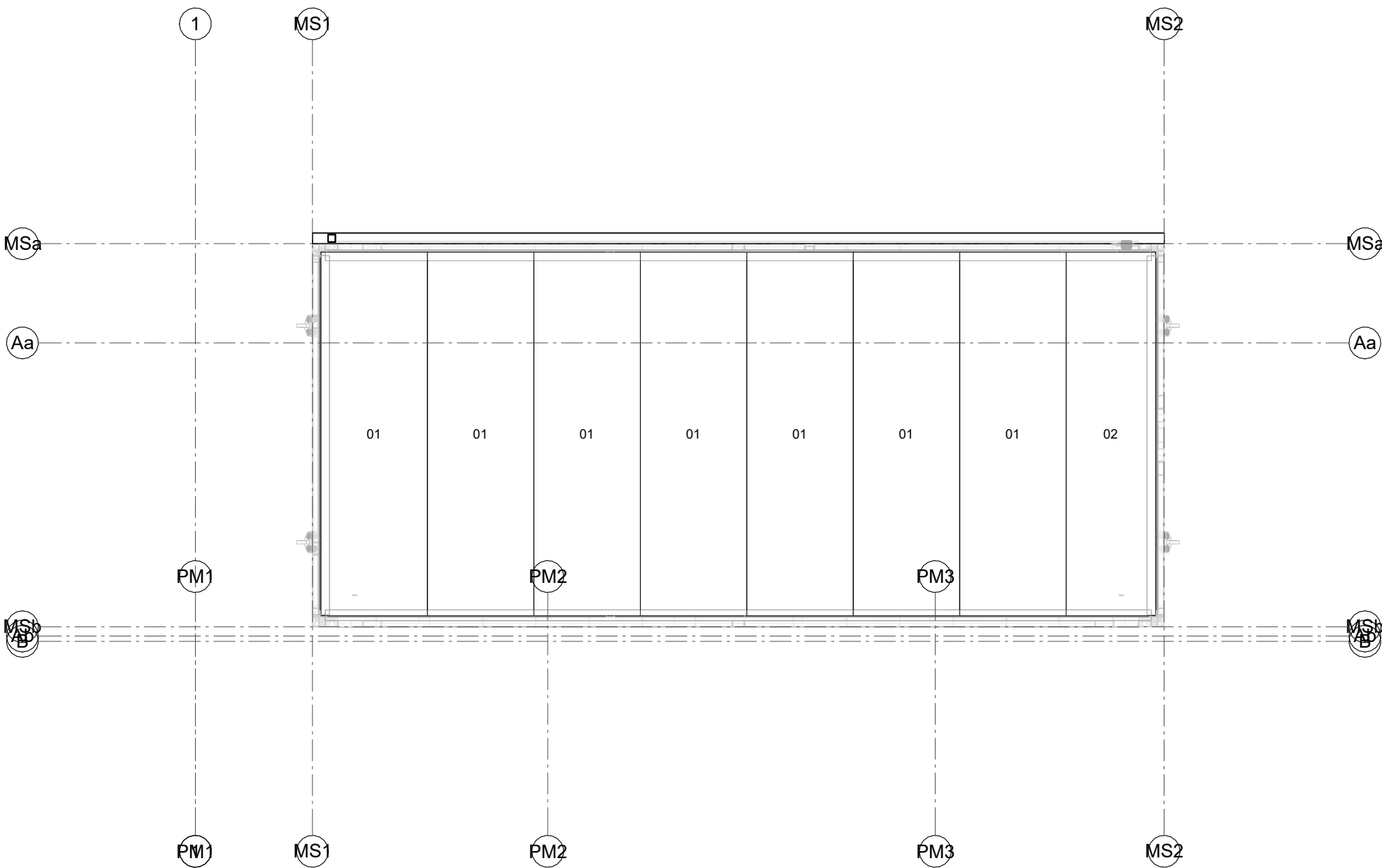
MS - Ceiling Layout - Ceiling Panel 100 Copy 1
