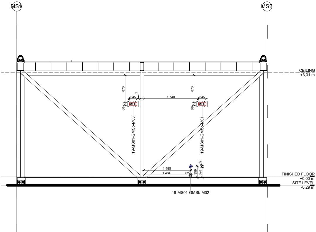
2 MS-PEN ELEVATION SOUTH 1 : 50
