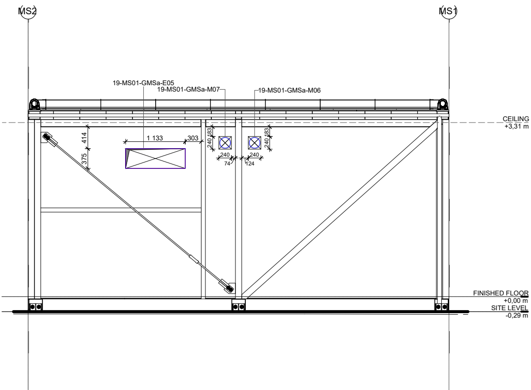
1 MS-PEN ELEVATION NORTH 1 : 50
