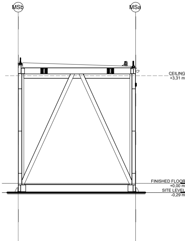
3 MS-PEN ELEVATION EAST 1 : 50
