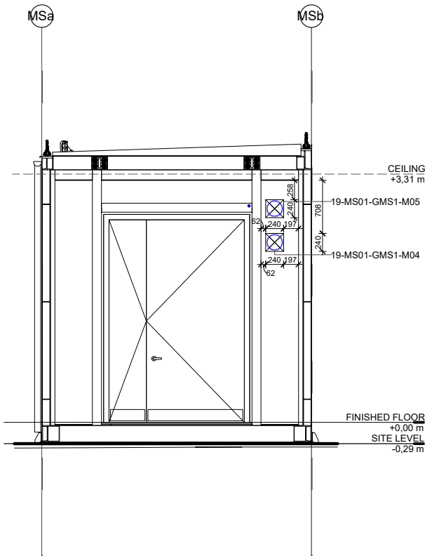
4 MS-PEN ELEVATION WEST 1 : 50
