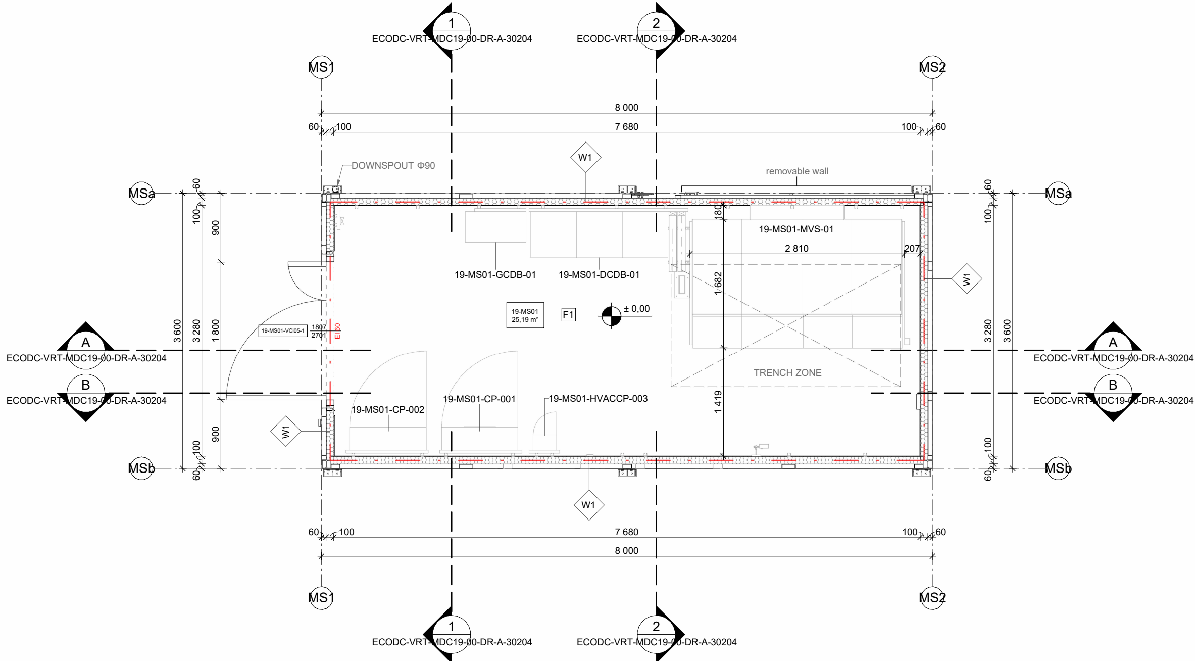
1 ARCHITECTURAL FLOOR PLAN - MS MODULE 1 : 50
