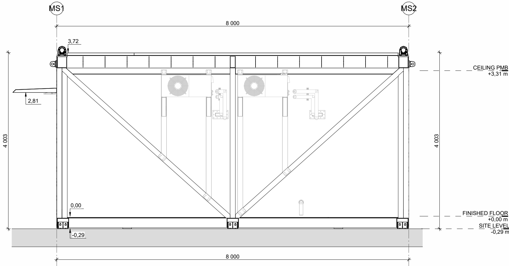
4 MS MODULE - ELEVATION SOUTH 1 : 50
