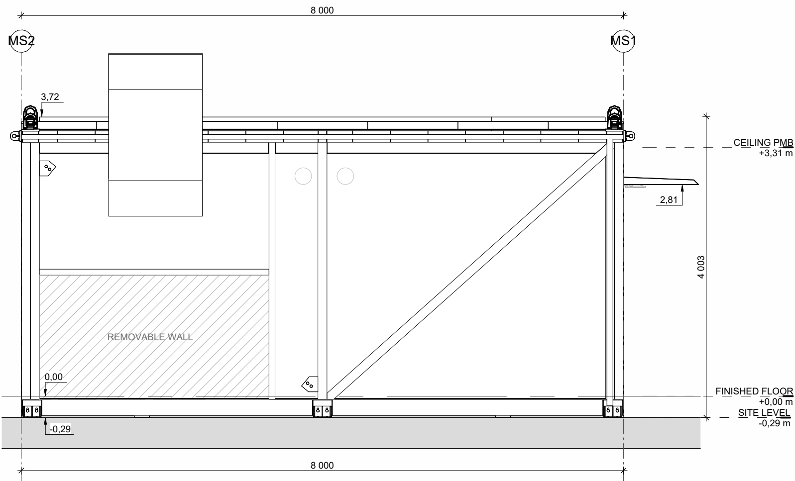
2 MS MODULE - ELEVATION NORTH 1 : 50
