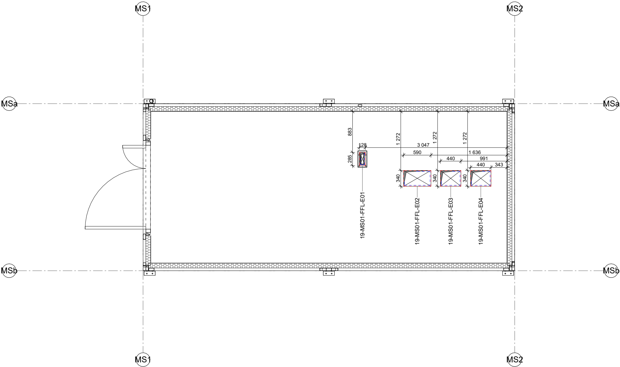
1 ARCHITECTURAL BUILDING PENETRATIONS – MS MODULE – FLOOR PLAN 1 : 50
