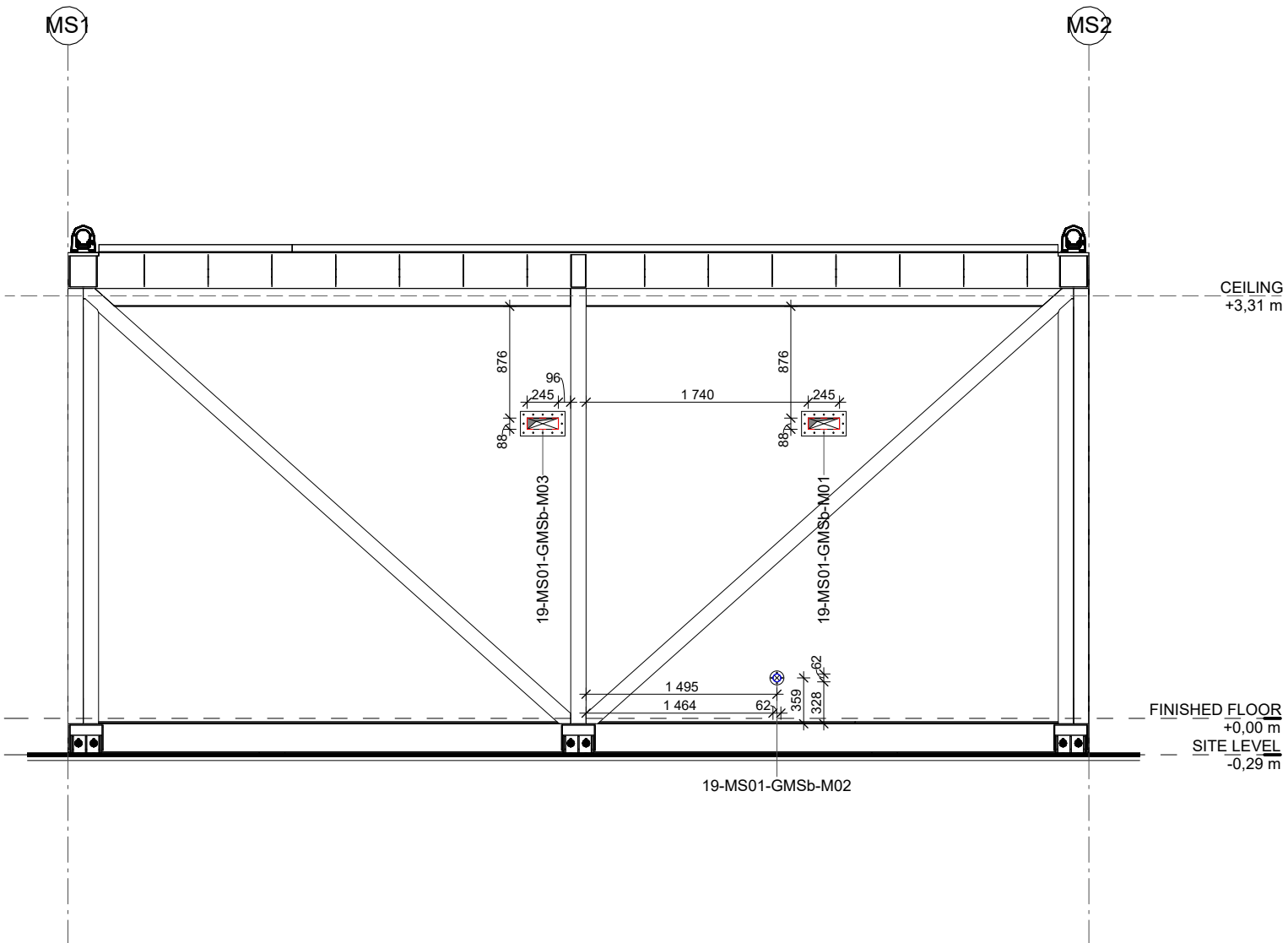
2 MS-PEN ELEVATION SOUTH 1 : 50
