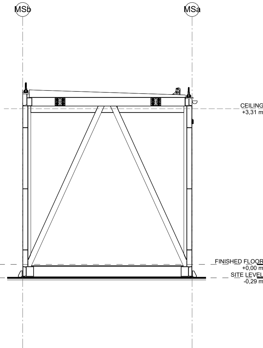
3 MS-PEN ELEVATION EAST 1 : 50
