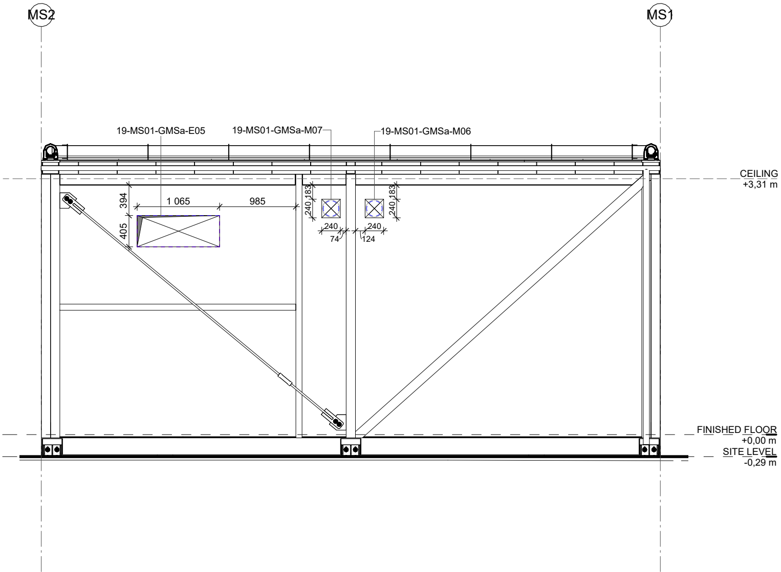
1 MS-PEN ELEVATION NORTH 1 : 50
