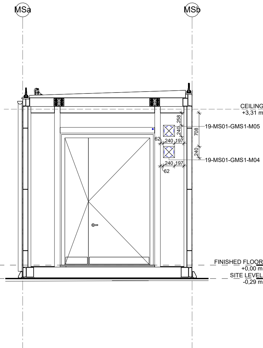
4 MS-PEN ELEVATION WEST 1 : 50
