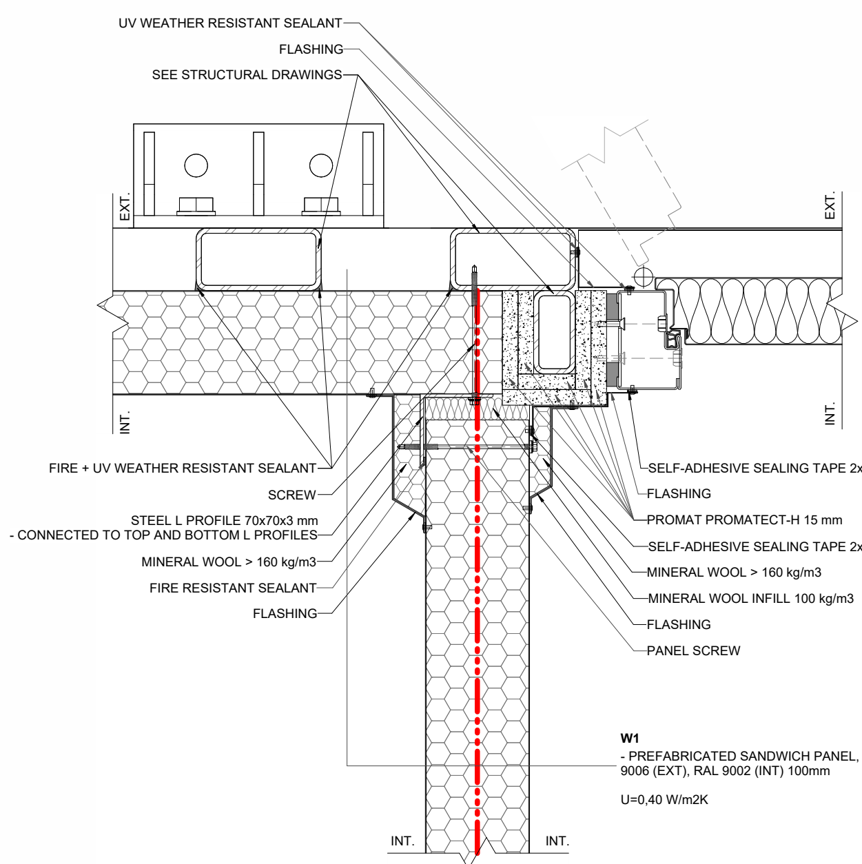
H02 MV - INT./EXT. WALL CONNECTION 1:5
