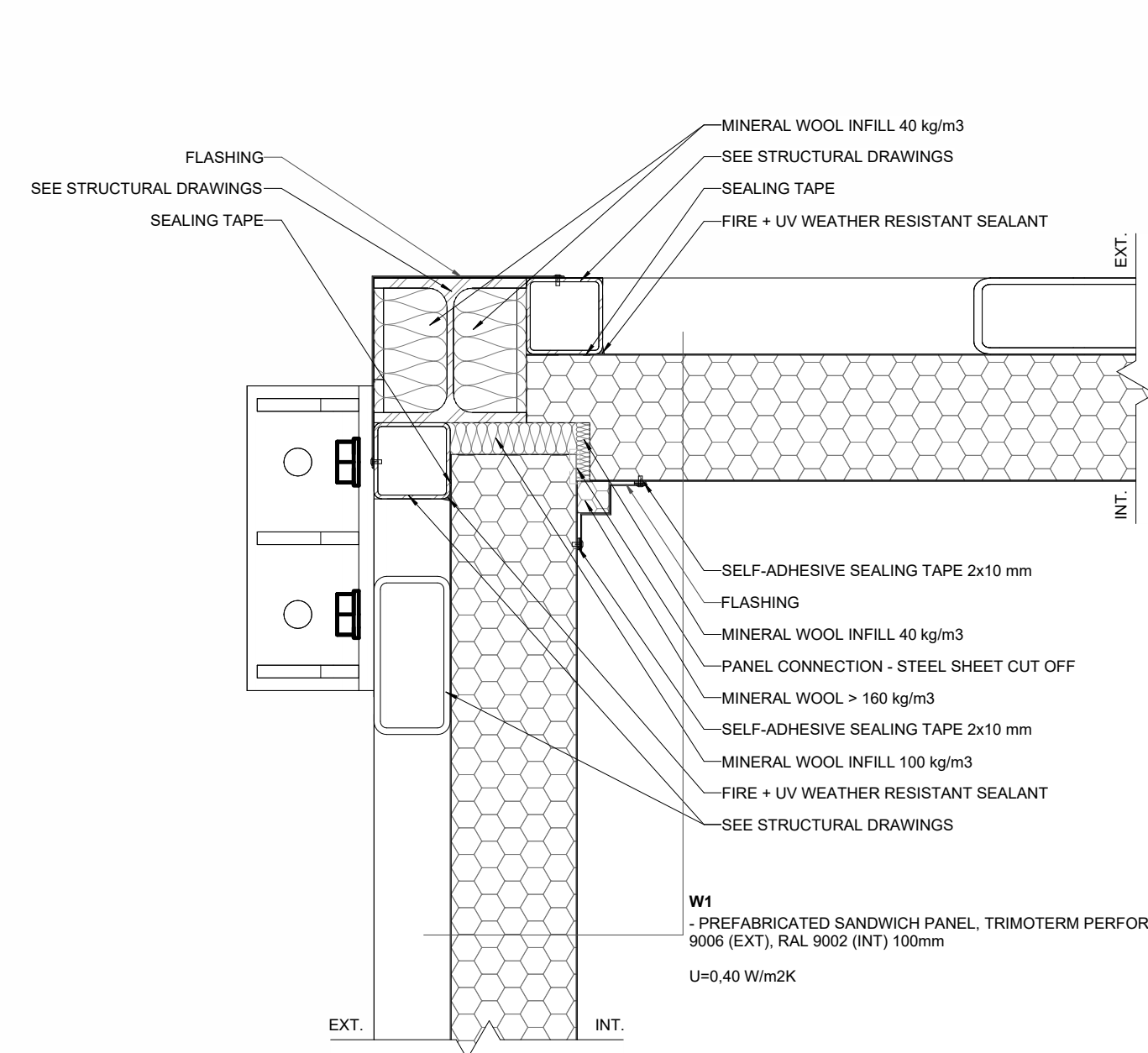
H01 MV/MS - MODULE CORNER 1:5
