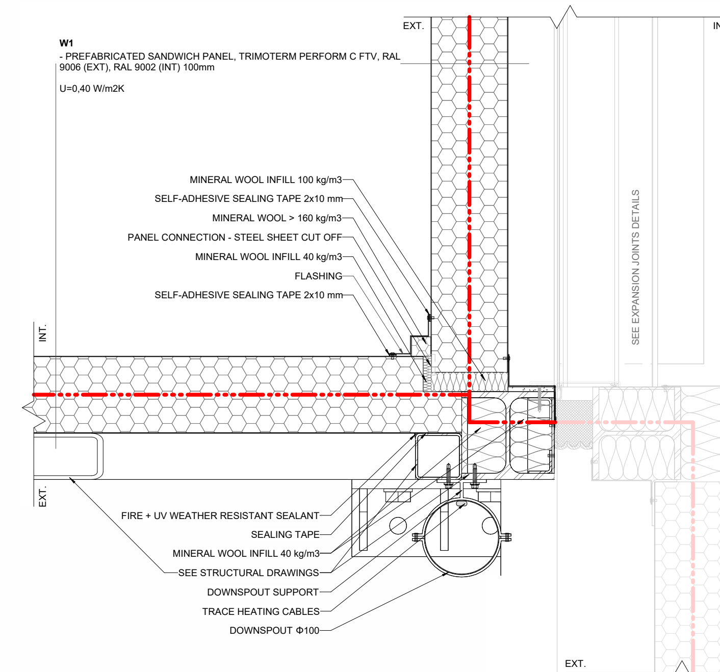
H10 PM - MODULE CORNER, RPP MODULE CONNECTION 1:5
