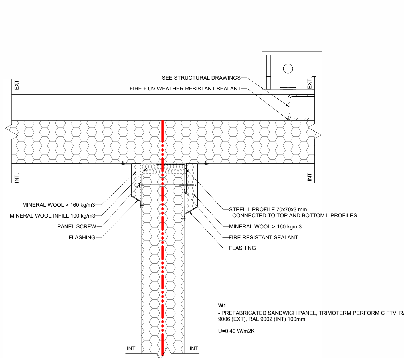
H03 MV - INT./EXT. WALL CONNECTION 1:5
