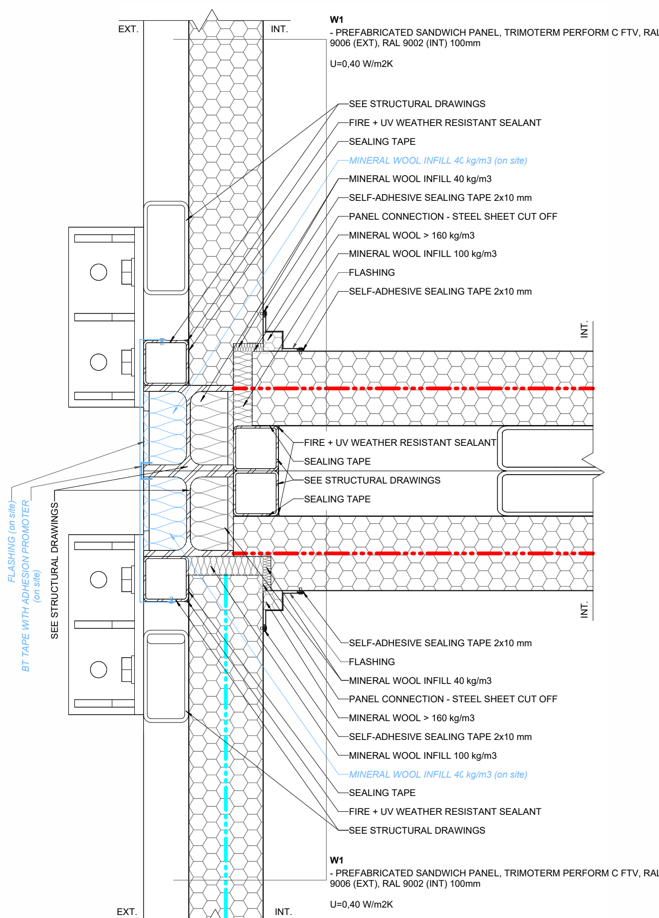
H05 PM/MV - MODULE CONNECTION 1:5
