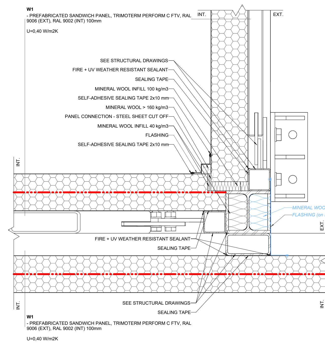
H07 MV - MODULE CORNER, PM MODULE CONNECTION 1:5
