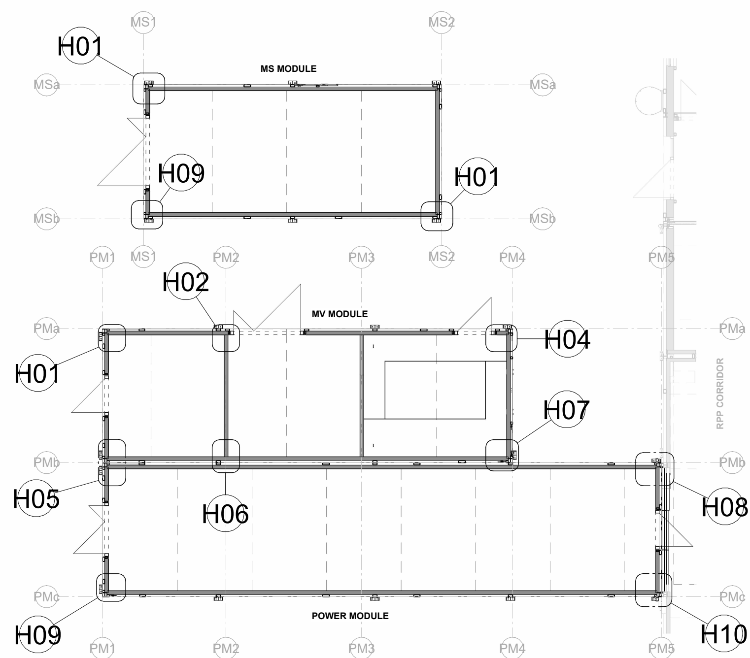
KEY PLAN - PM/MV/MS MODULE DETAIL POSITIONS - HORIZONTAL VIEWS
