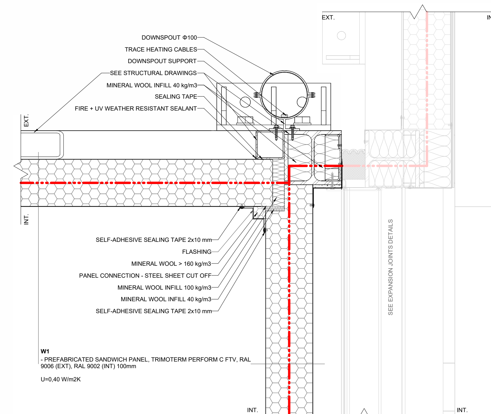
H08 PM - MODULE CORNER, RPP MODULE CONNECTION 1:5
