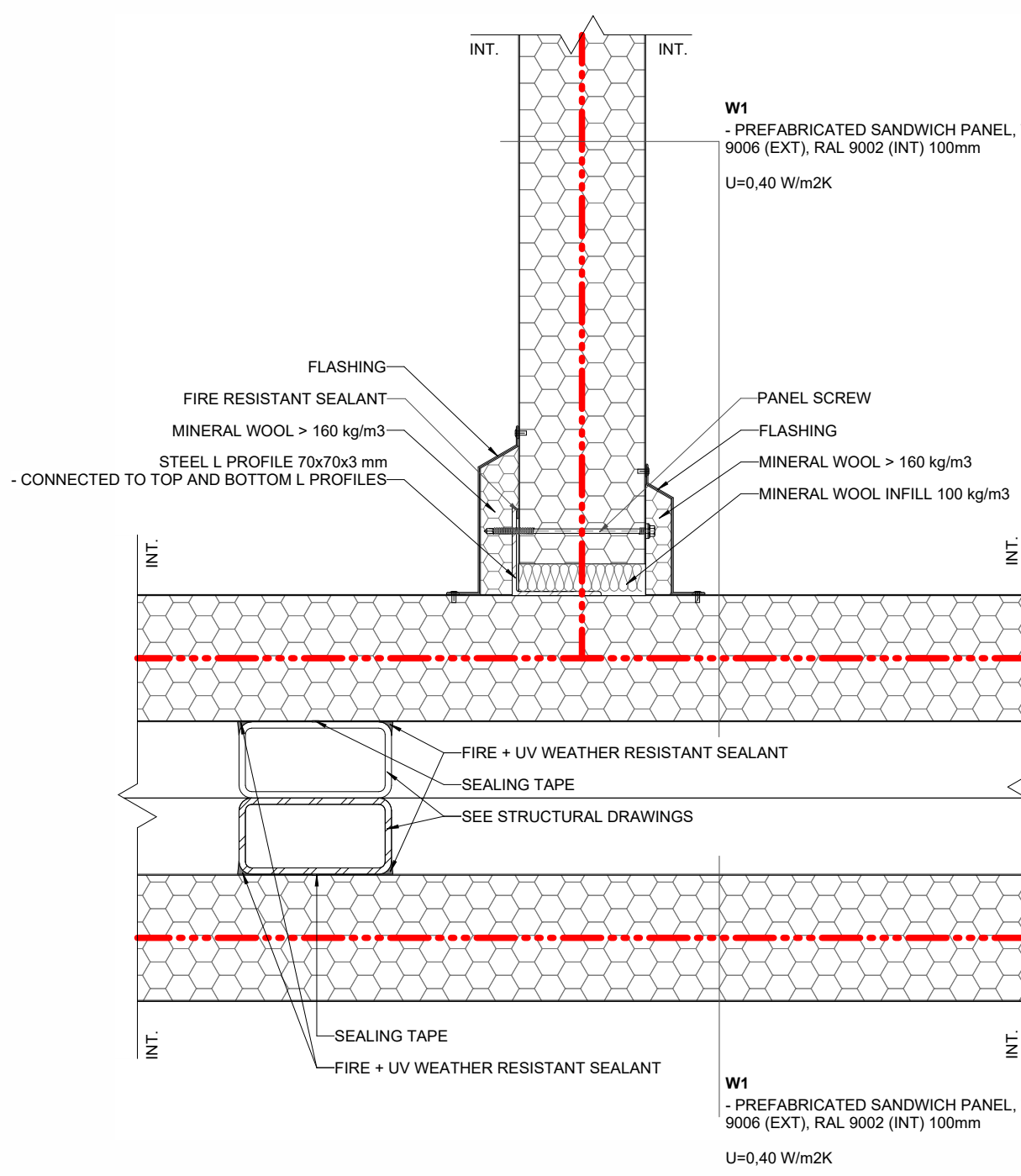
H06 MV - INT./EXT. WALL CONNECTION 1:5
