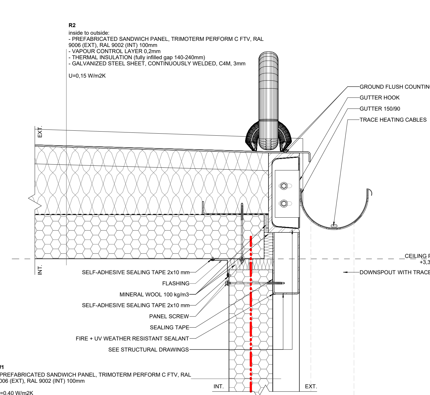
V09 PM/MV/MS - EXT. WALL/ROOF CONNECTION 1:5
