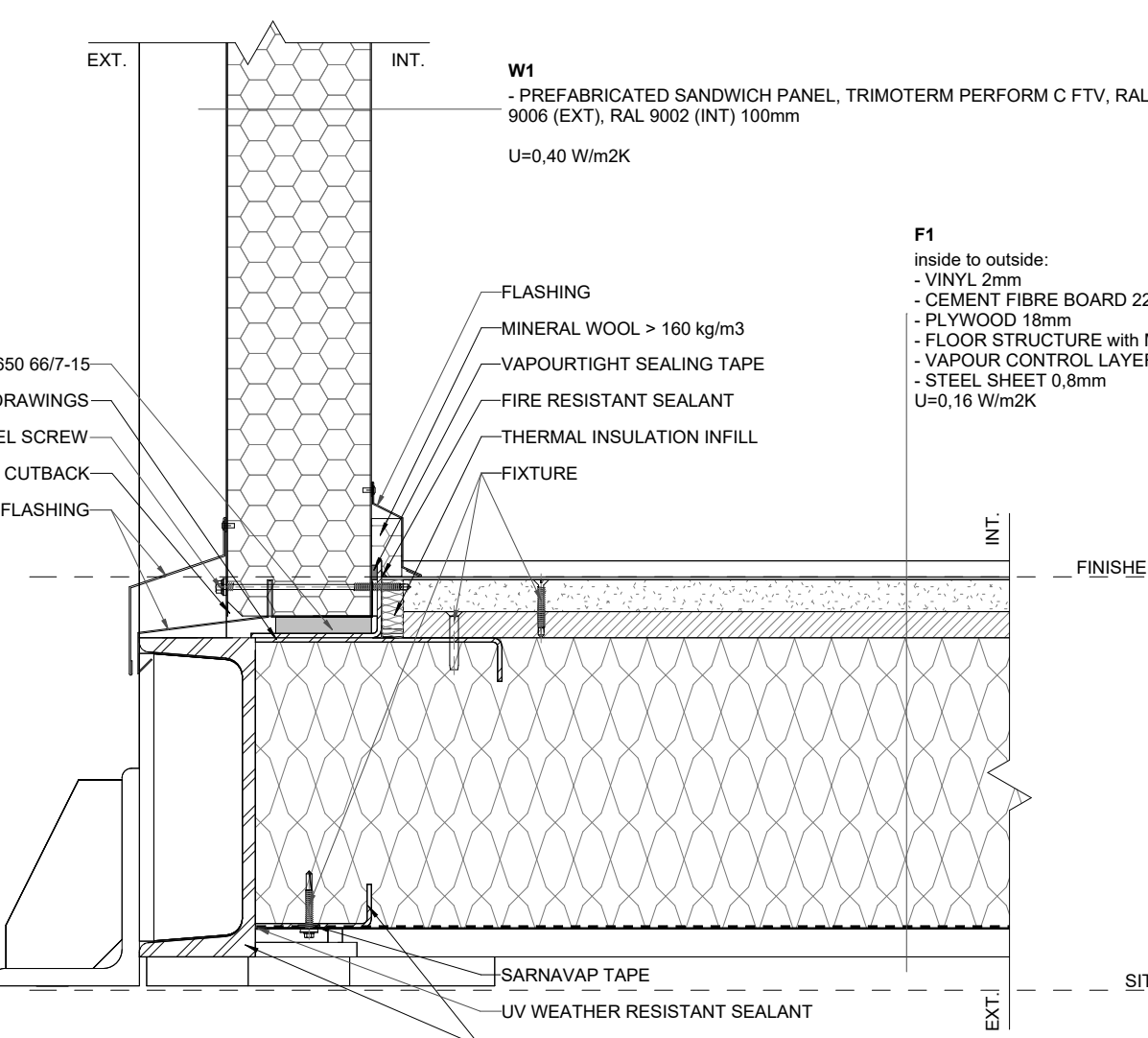
V02 PM/MV/MS - EXT. WALL/FLOOR CONNECTION 1:5
