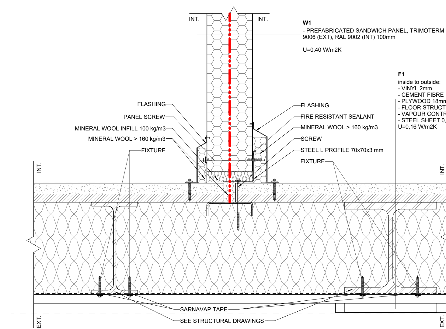
V06 MV - INT. WALL/FLOOR CONNECTION 1:5
