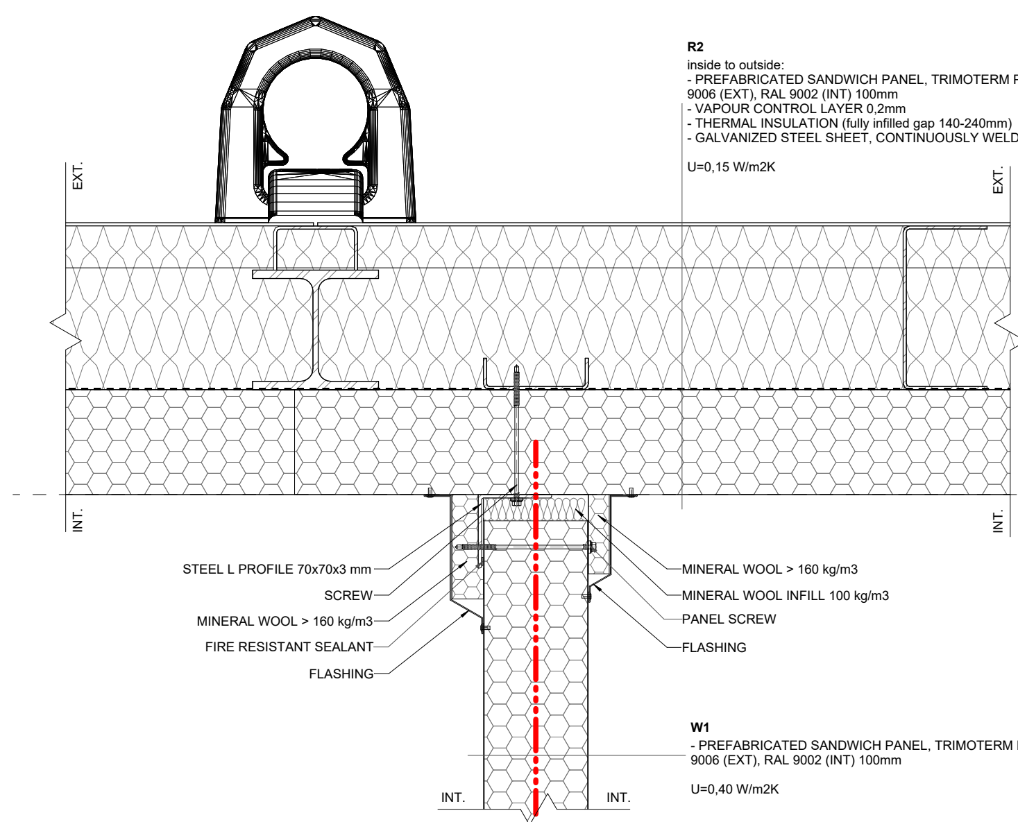
V03 MV - INT. WALL/ROOF CONNECTION 1:5
