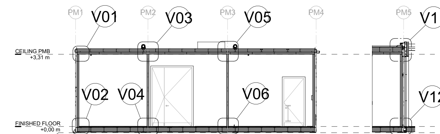
LONGITUDINAL SECTION KEY PLAN - PM/MV/MS MODULE DETAIL POSITIONS - VERTICAL VIEWS
