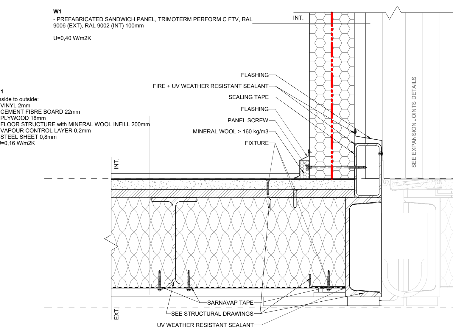
V12 PM - RPP MODULE CONNECTION-FLOOR 1:5
