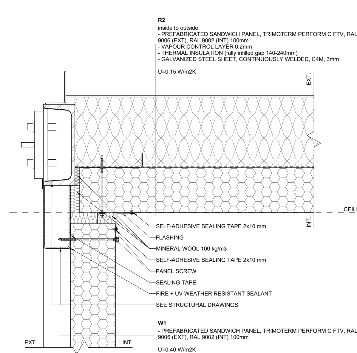
V01 PM/MV/MS - EXT. WALL/ROOF CONNECTION 1:5
