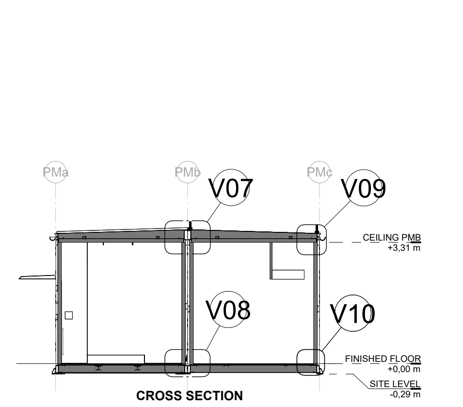
CROSS SECTION KEY PLAN - PM/MV/MS MODULE DETAIL POSITIONS
