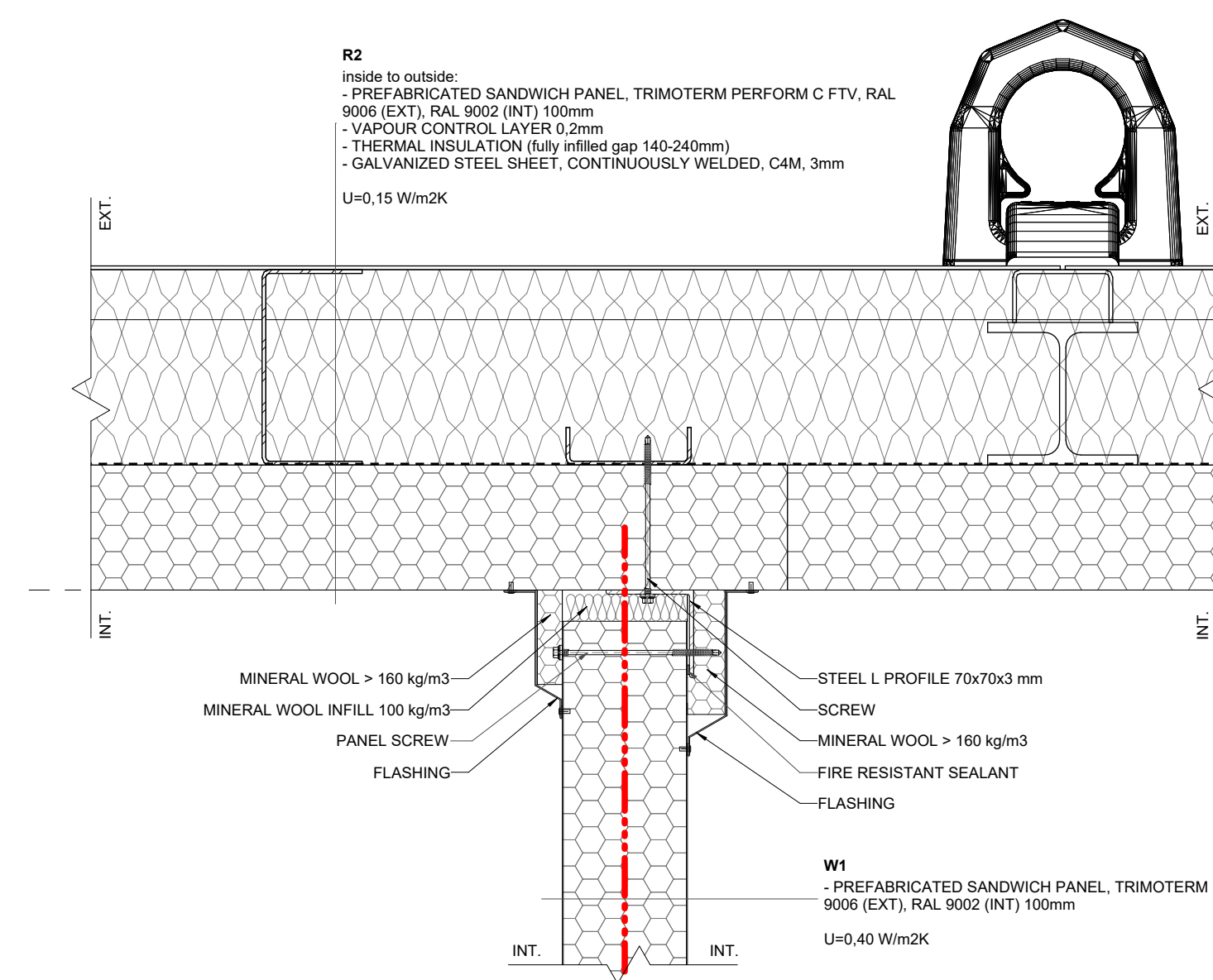
V05 MV - INT. WALL/ROOF CONNECTION 1:5
