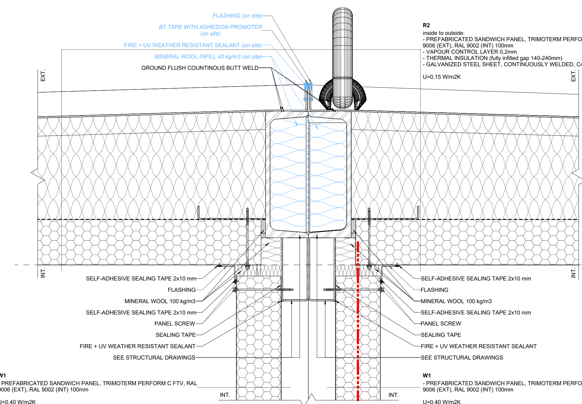
V07 PM/MV - MODULE CONNECTION-ROOF 1:5
