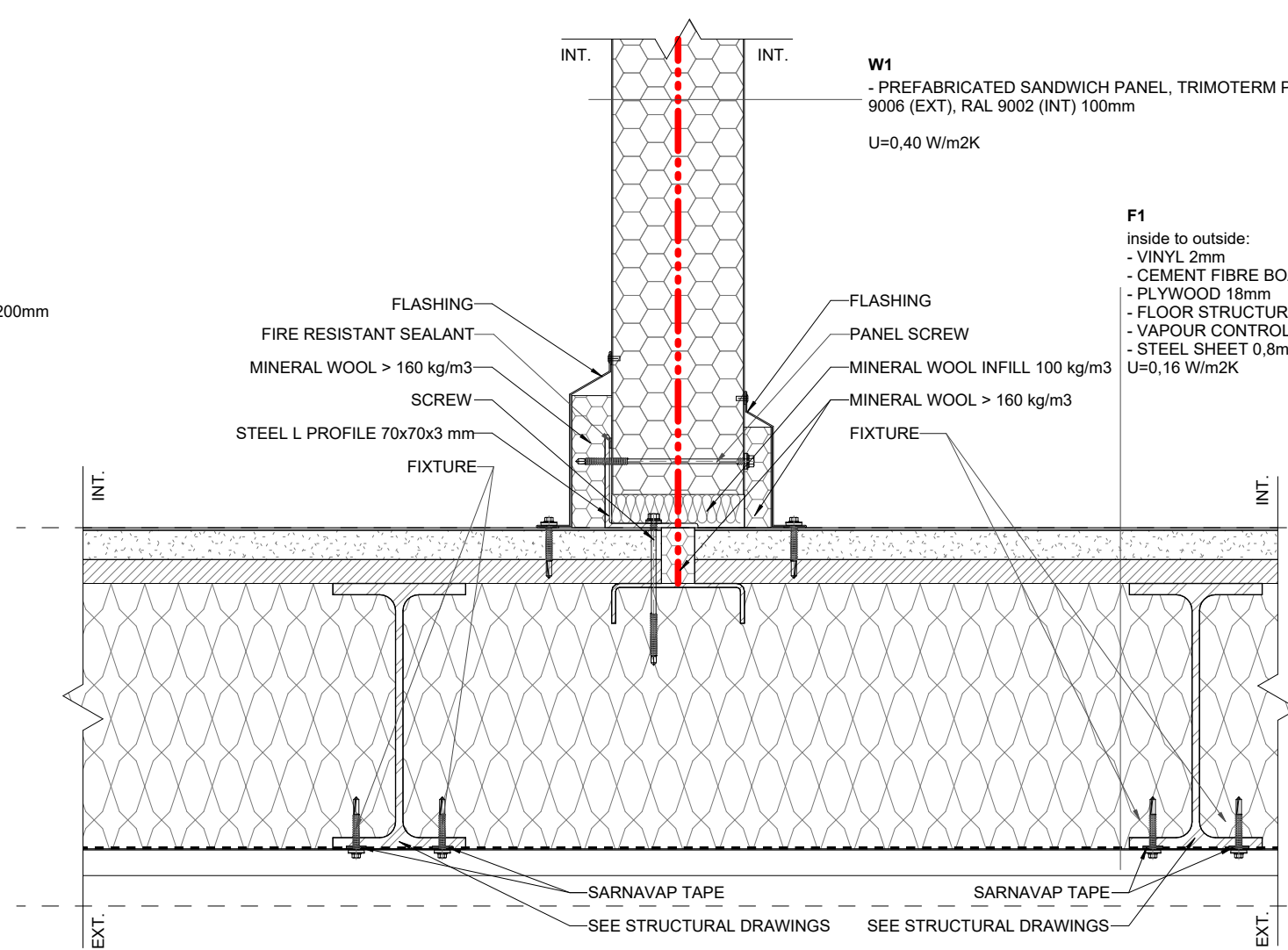
V04 MV - INT. WALL/FLOOR CONNECTION 1:5
