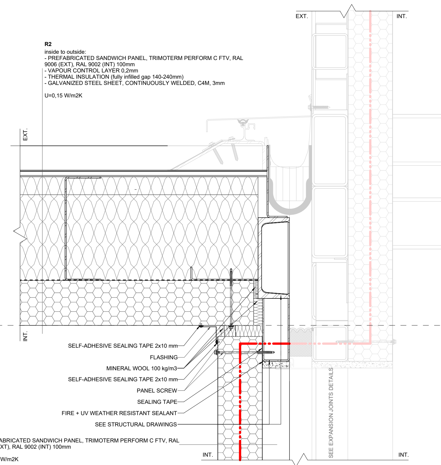
V11 PM - RPP MODULE CONNECTION-ROOF 1:5
