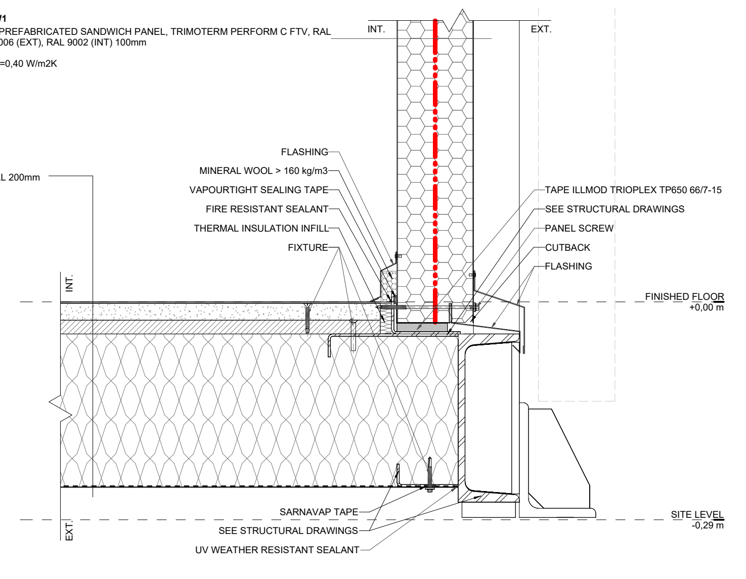
V10 PM/MV/MS - EXT. WALL/FLOOR CONNECTION 1:5
