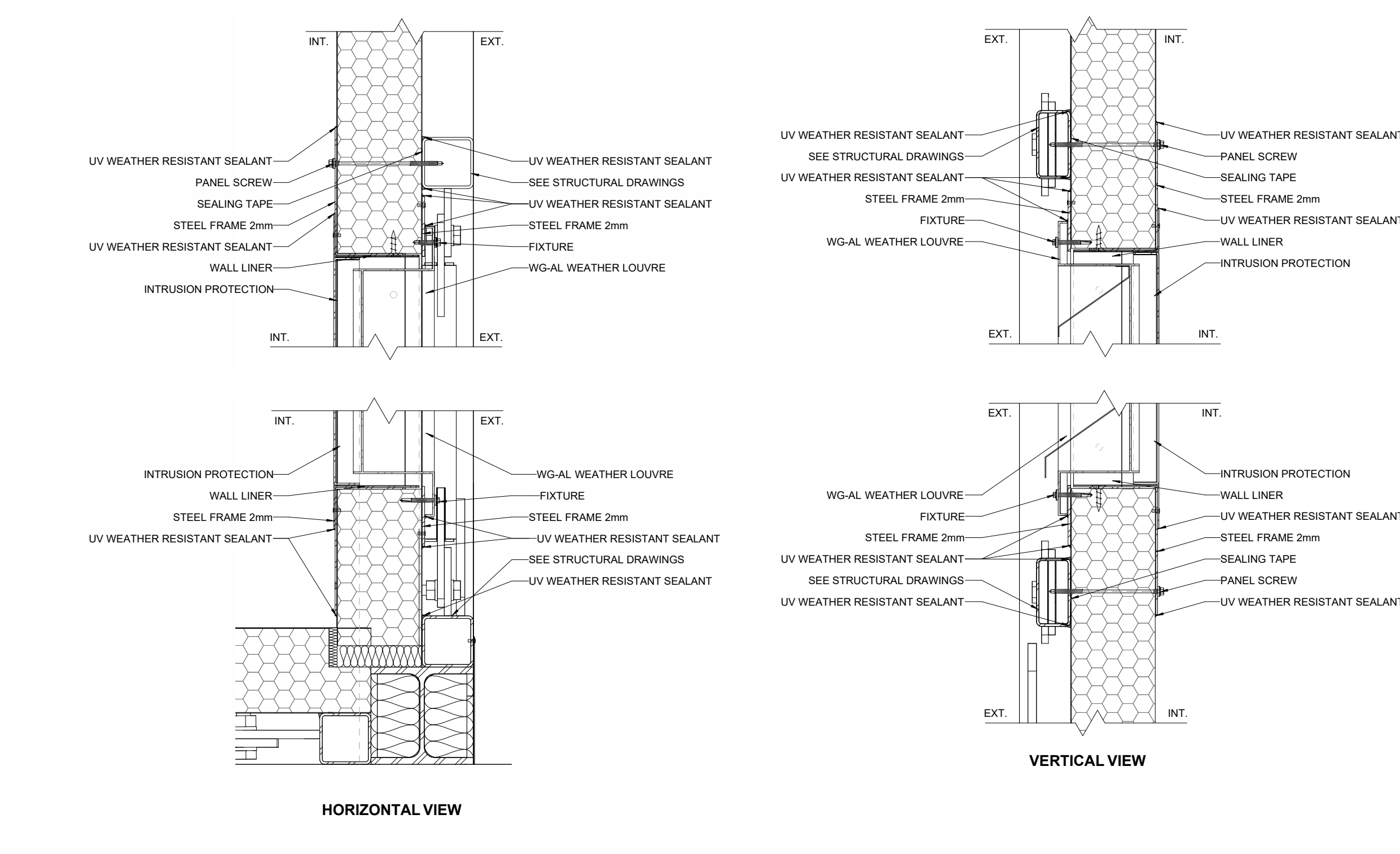
P11b WG-AL WEATHER LOUVRE 1:5
