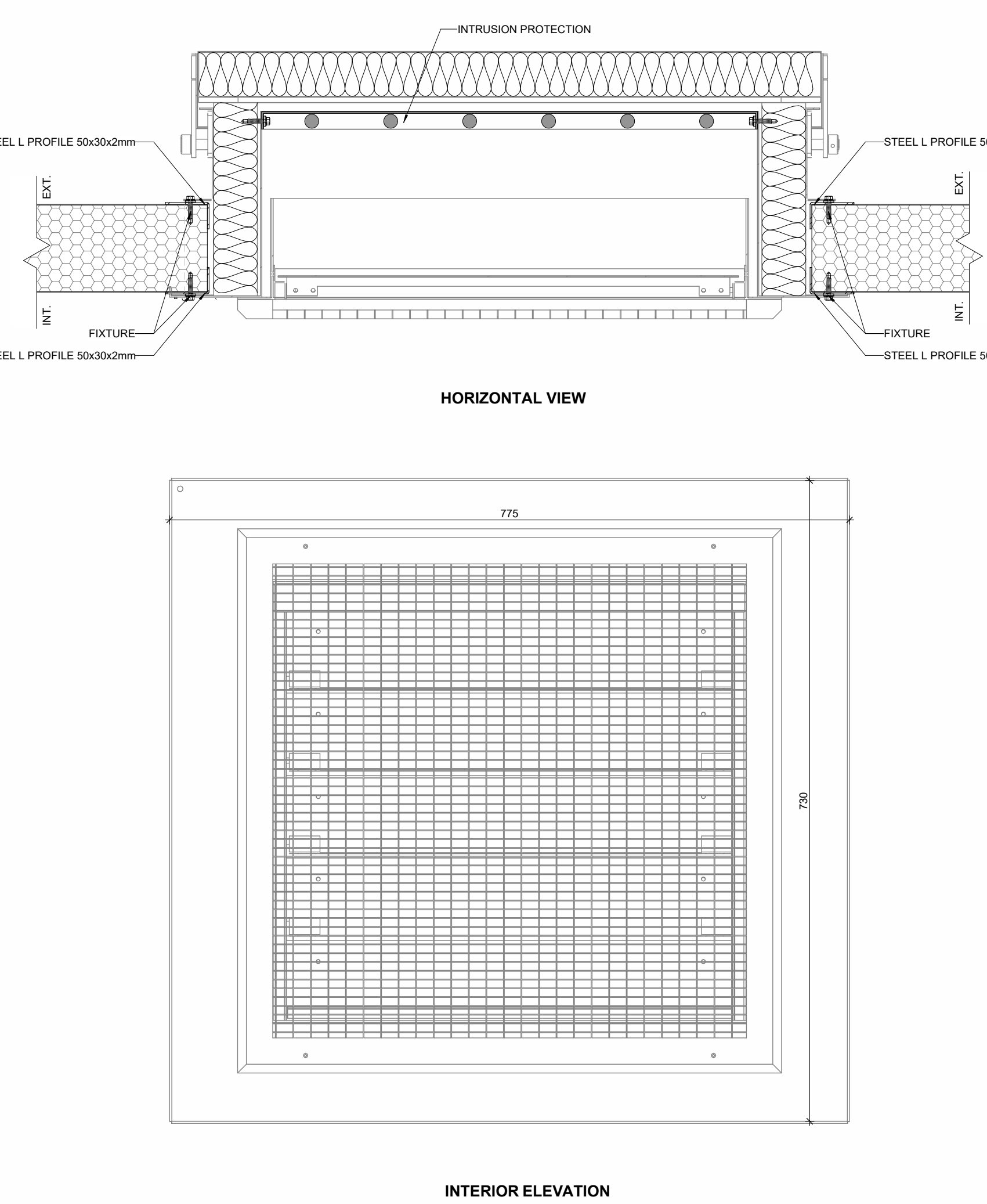
INTERIOR ELEVATION
