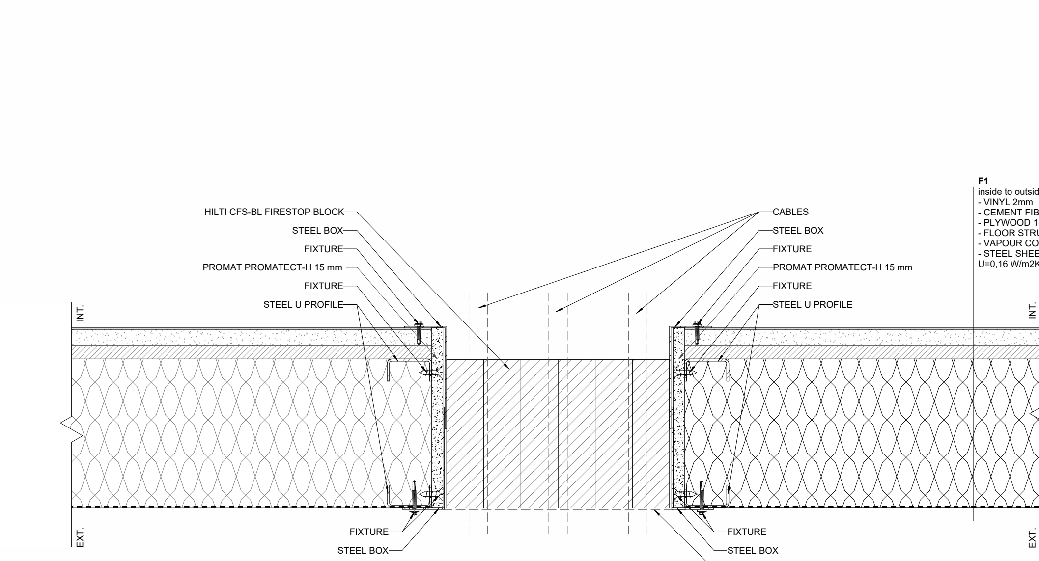
P15 HILTI CFS-BL FIRESTOP BLOCKS - FLOOR 1:5
