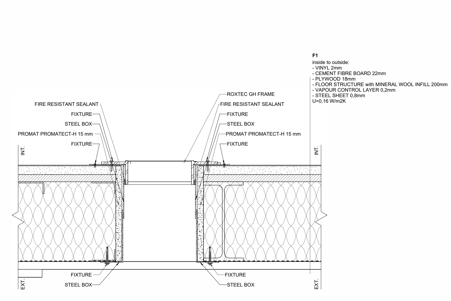
P03 ROXTEC GH - FLOOR 1:5
