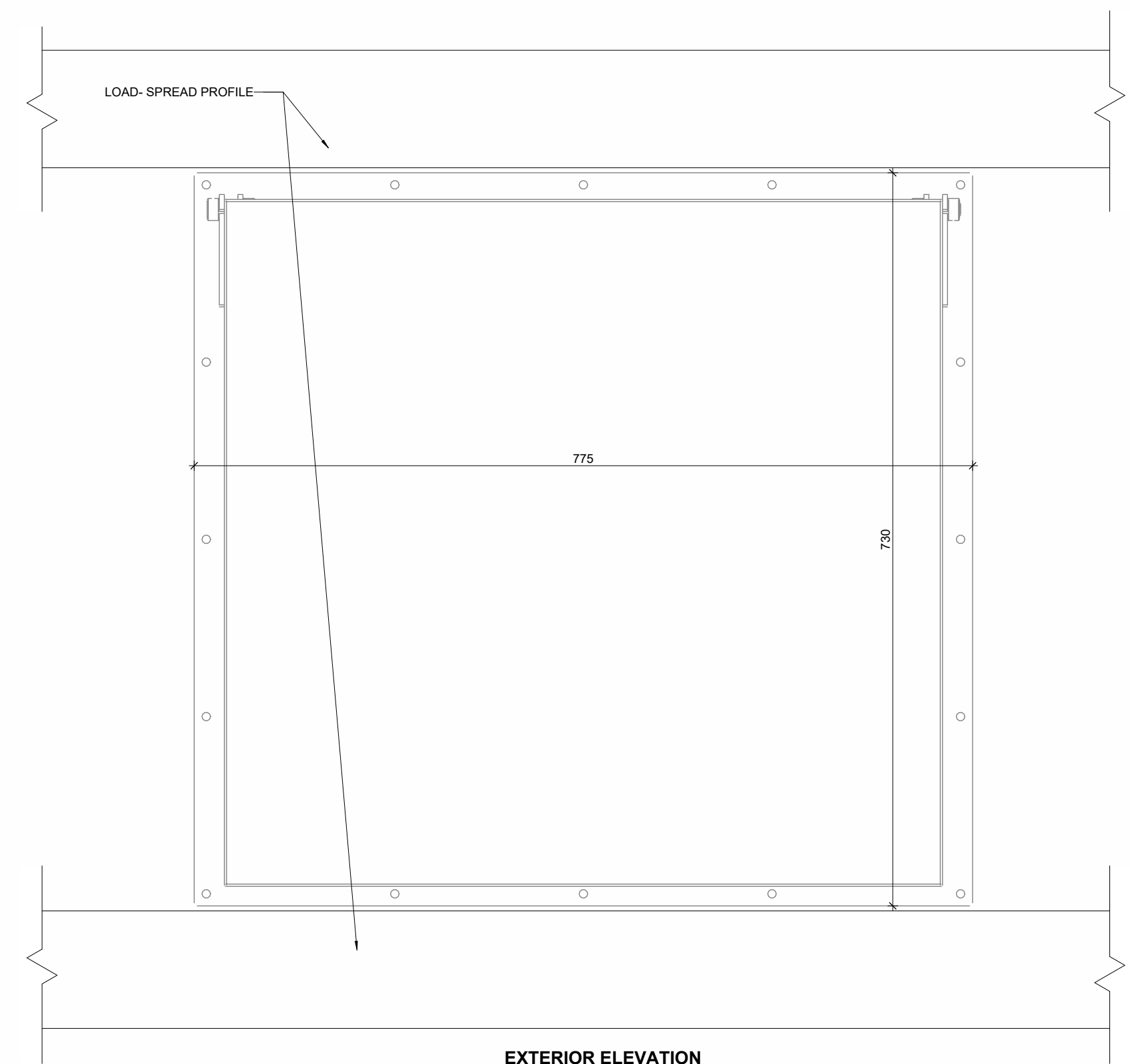
EXTERIOR ELEVATION
