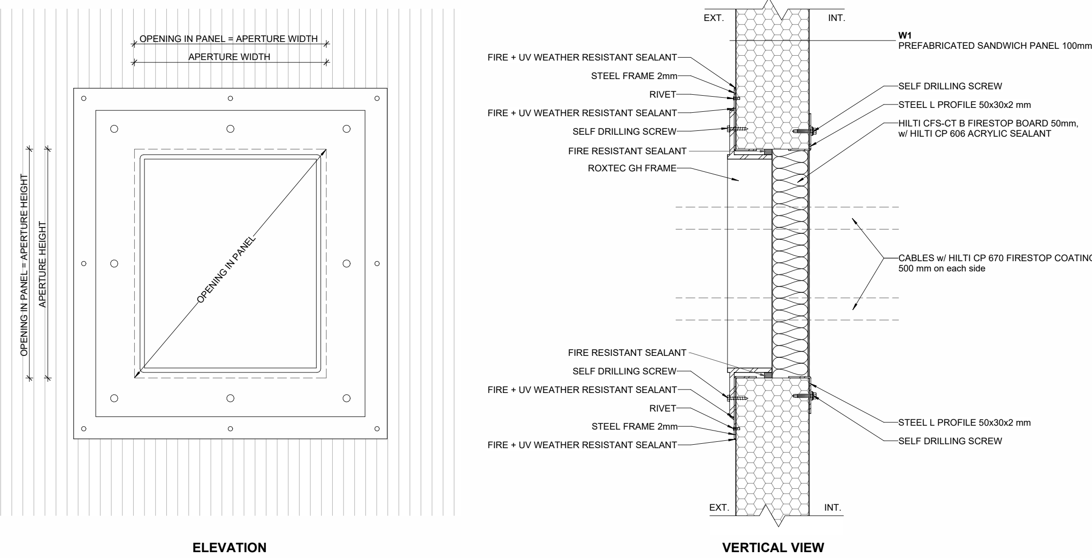
P01 ROXTEC GH - EXTERIOR WALL 100 mm 1:5
