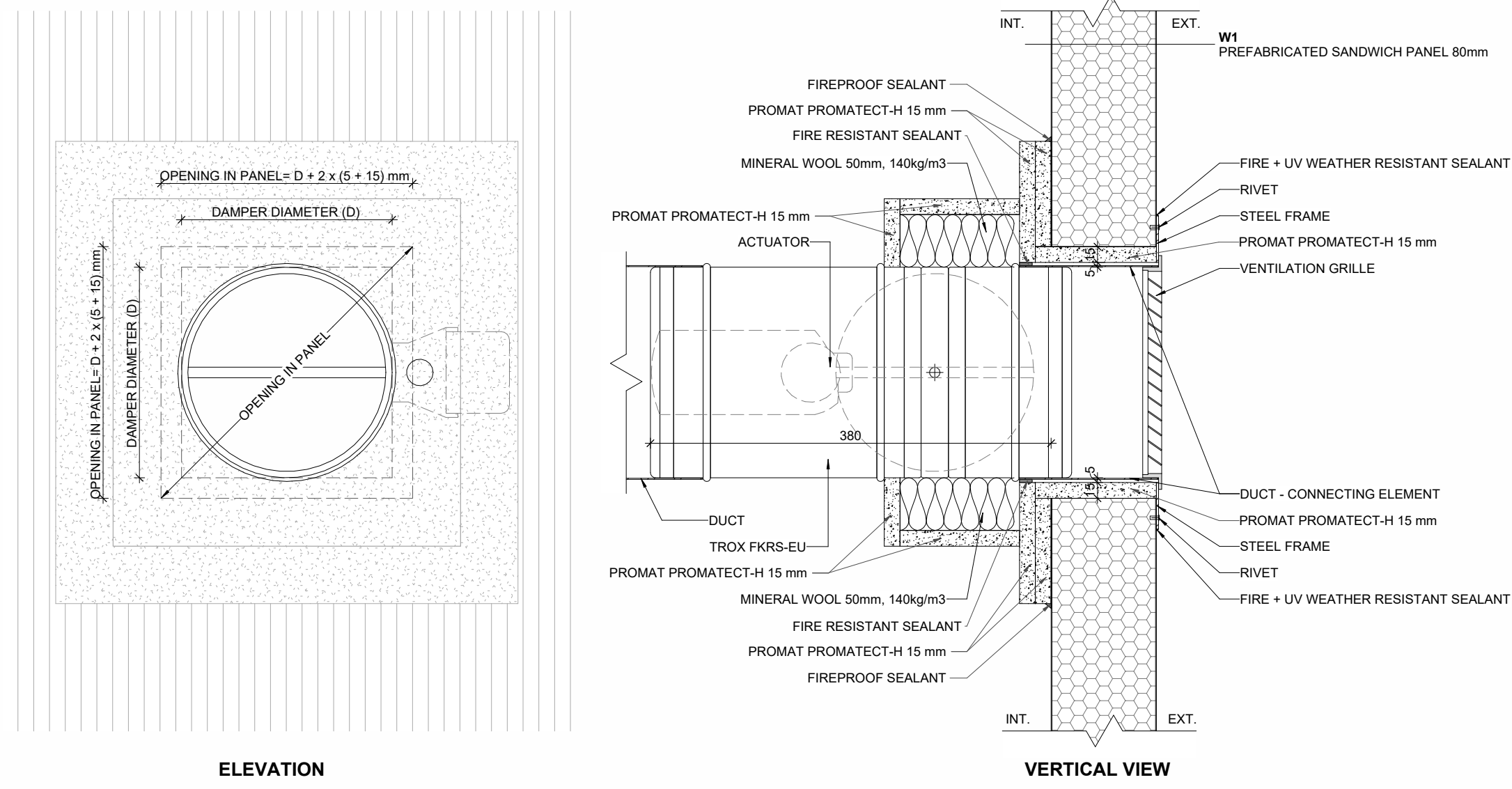
P06 TROX FKRS-EU 1:5
