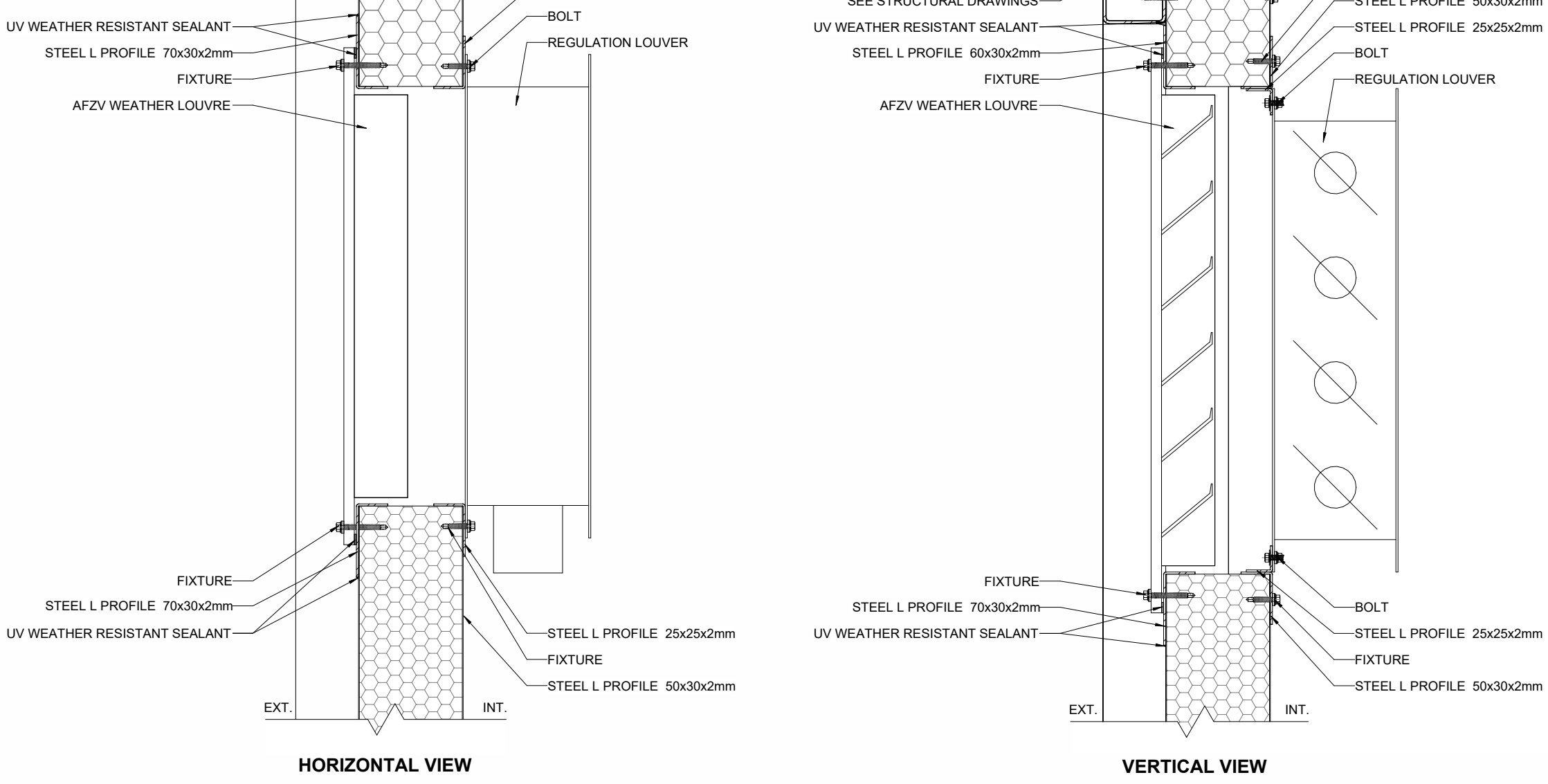
P11 AFZV WEATHER LOUVRE + REGULATION LOUVRE 1:5
