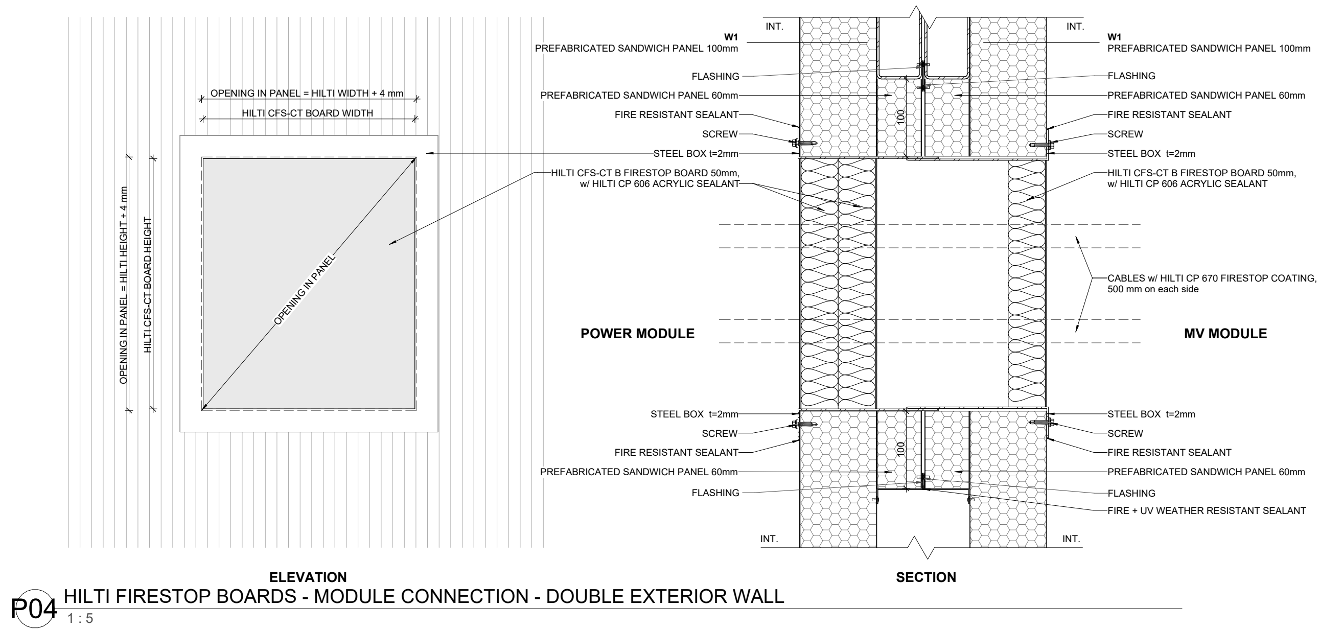
P04 HILTI FIRESTOP BOARDS - MODULE CONNECTION - DOUBLE EXTERIOR WALL 1:5
