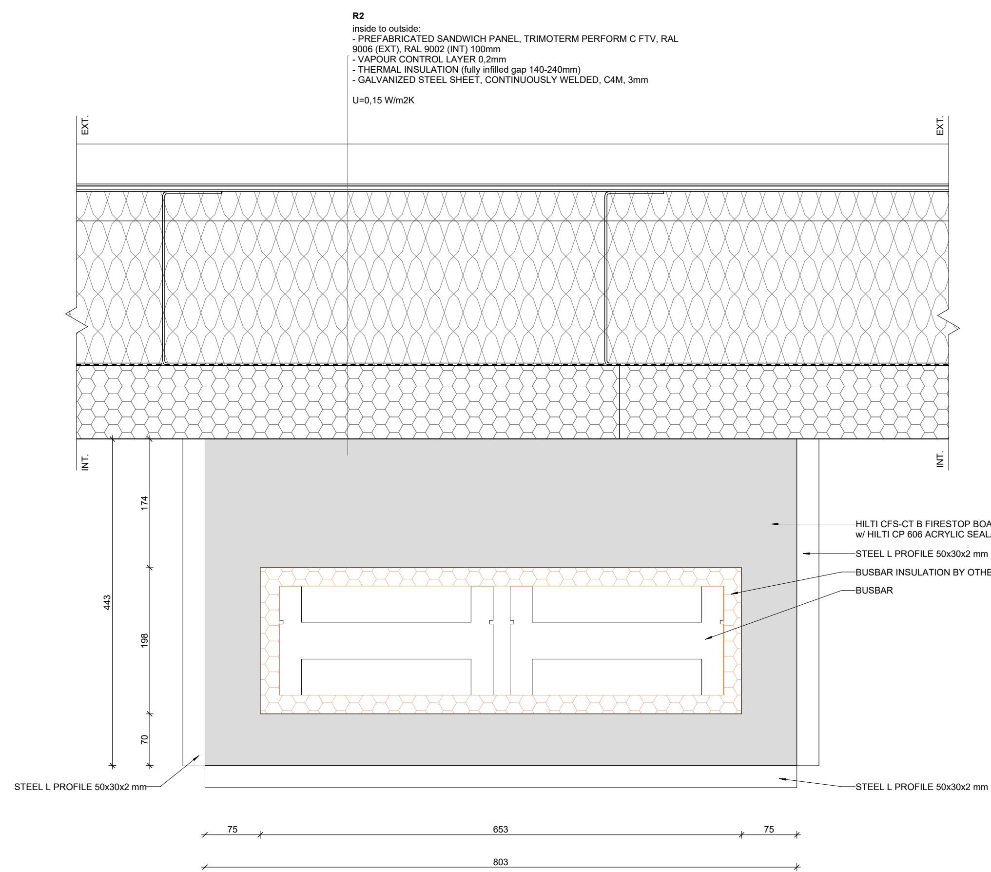
P09 PM BUSBAR-DOUBLE EXT. WALL 1:5
