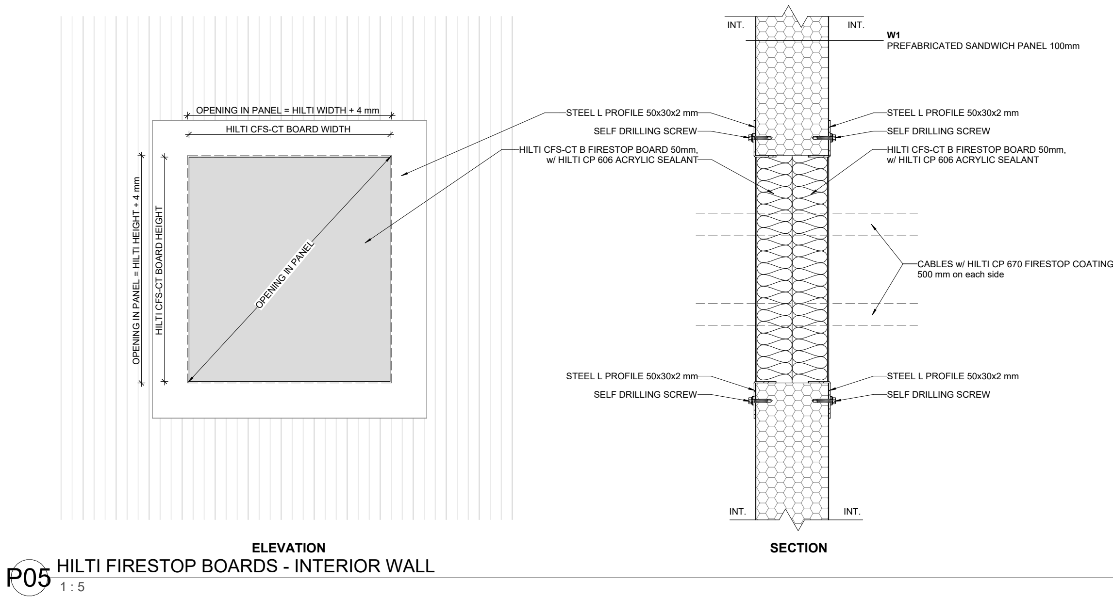
P05 HILTI FIRESTOP BOARDS - INTERIOR WALL 1:5
