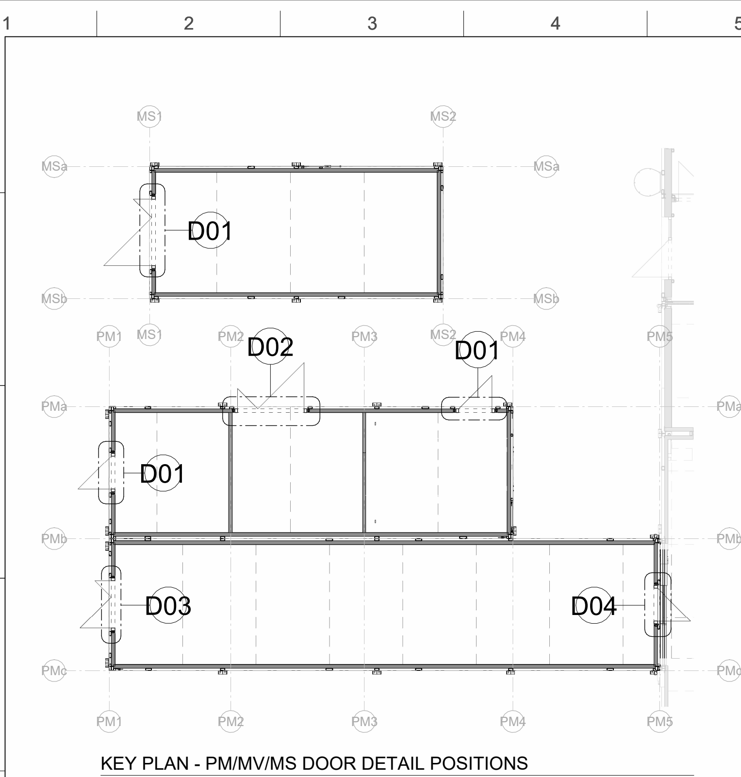
KEY PLAN - PM/MV/MS DOOR DETAIL POSITIONS
