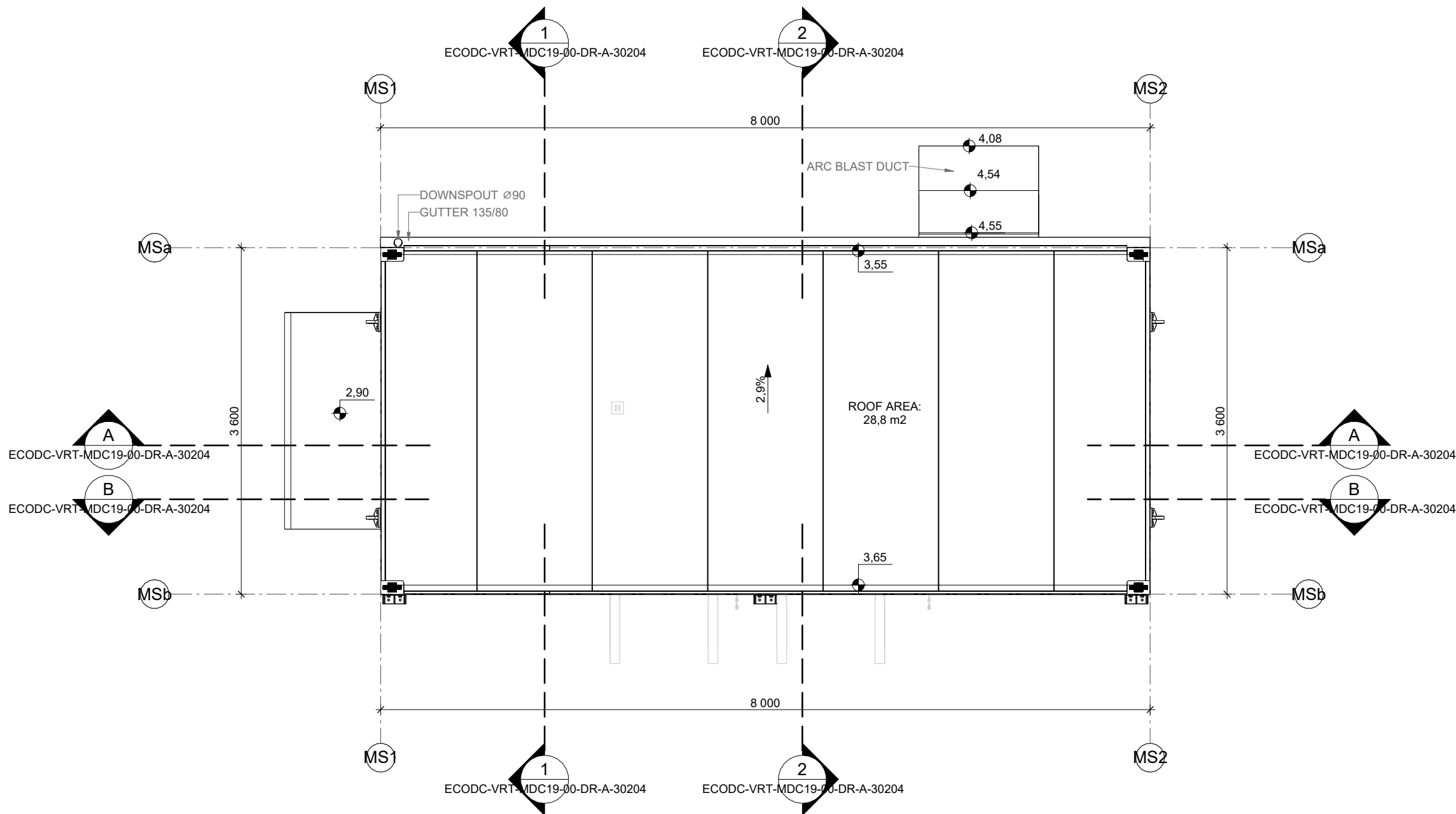
1 ARCHITECTURAL ROOF PLAN - MS MODULE 1 : 50
