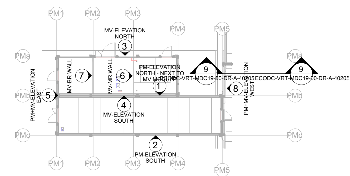
KEYPLAN – POWER MODULE – PEN ELEVATION POSITIONS
