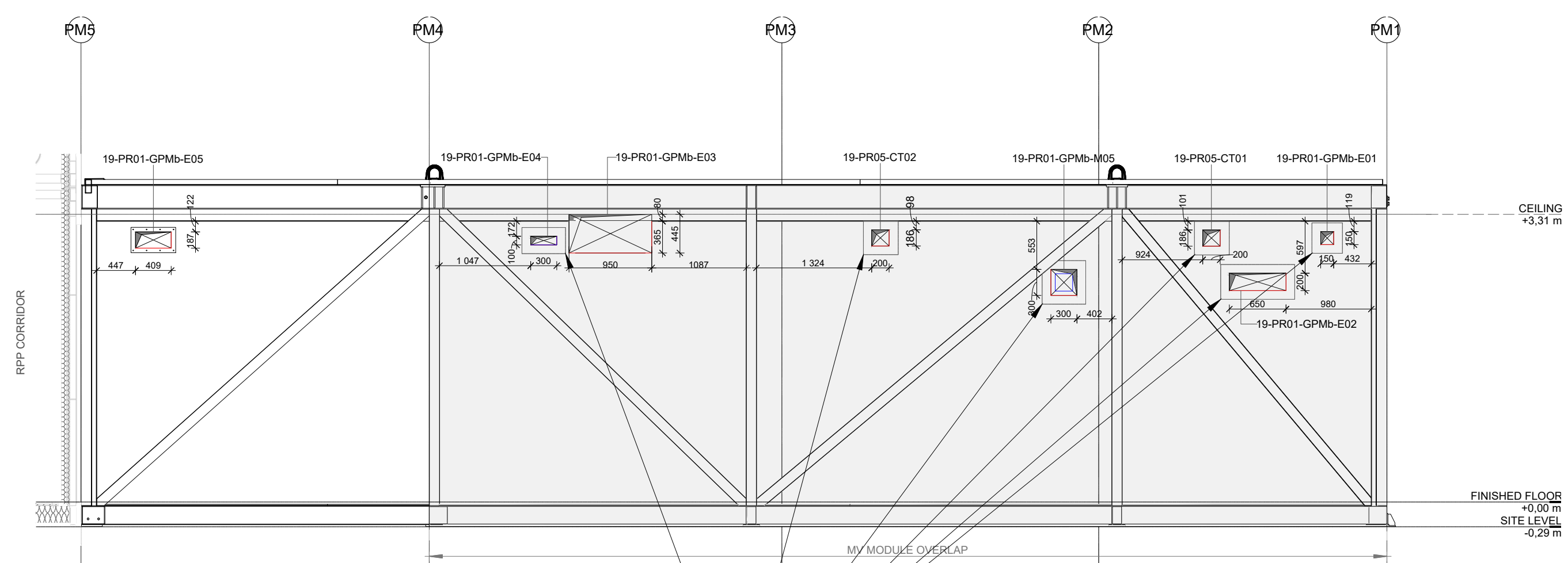
1 PM-ELEVATION NORTH - NEXT TO MV MODULE 1:50
