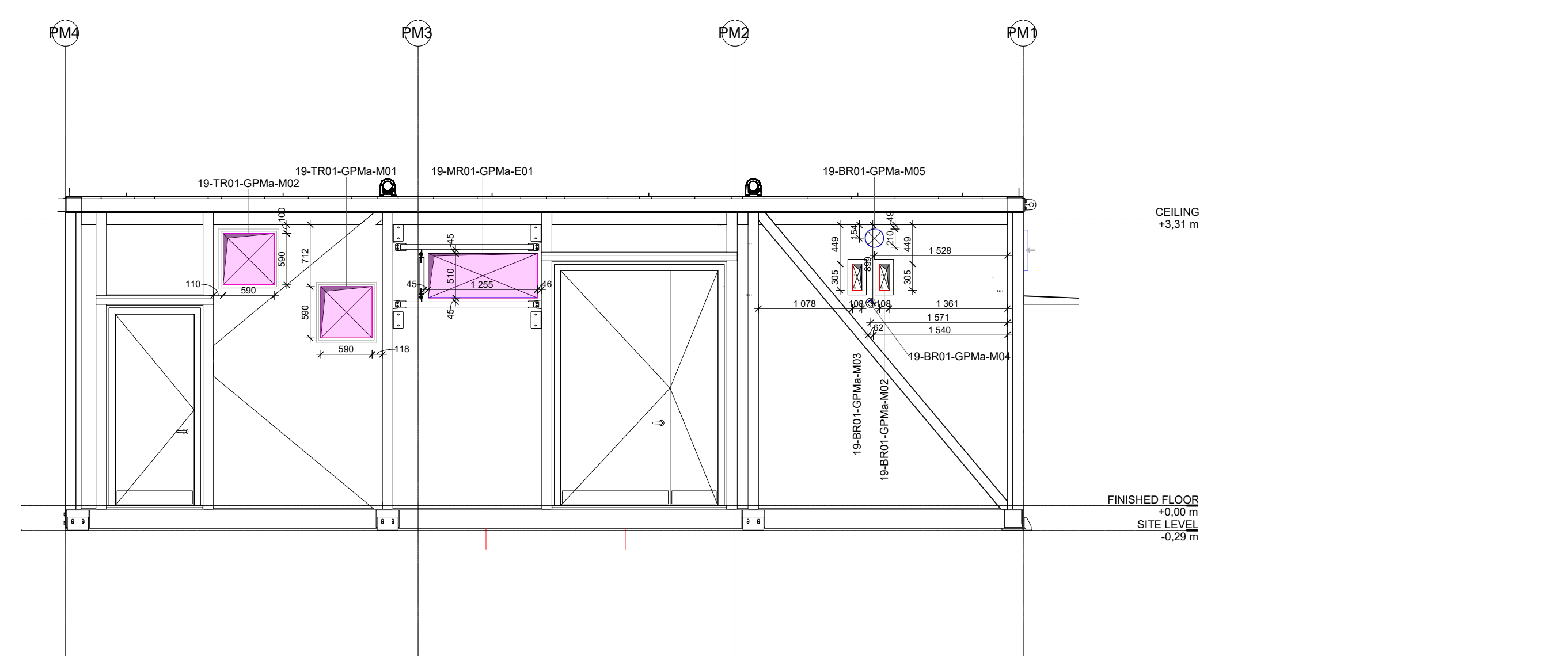
3 MV-ELEVATION NORTH 1:50
