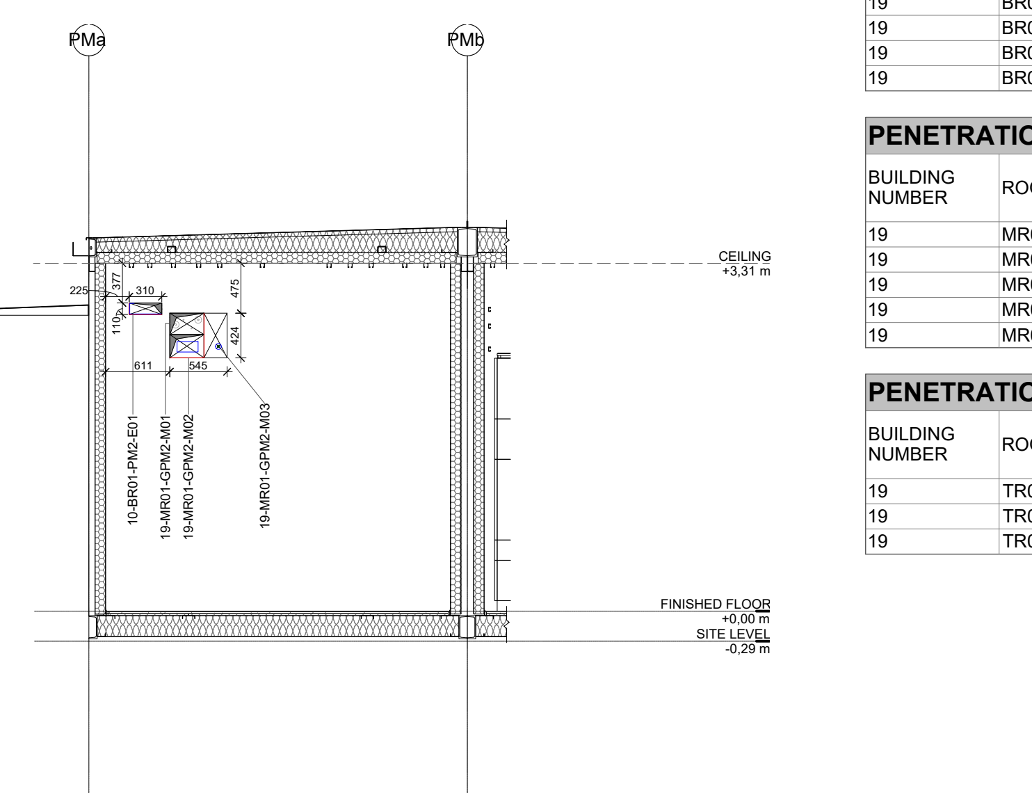
7 MV-BR WALL 1:50
