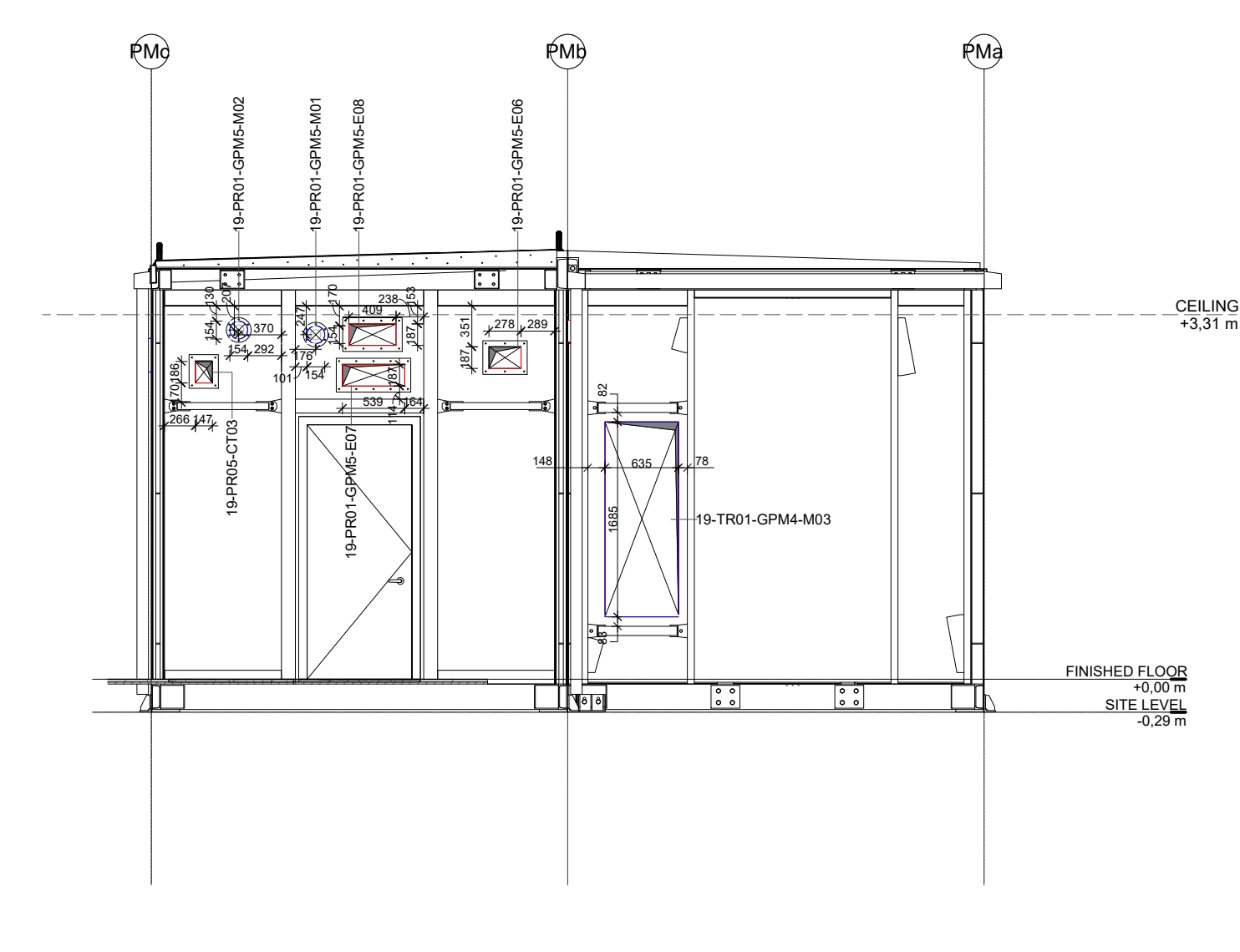
8 PM+MV-ELEVATION WEST 1:50
