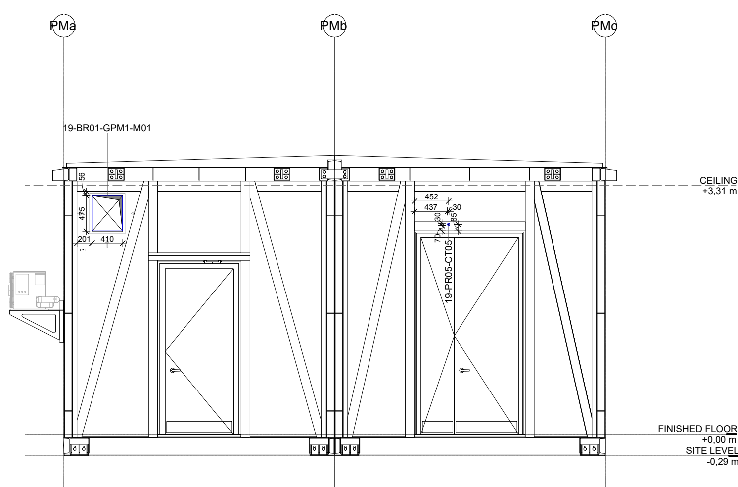
5 PM+MV-ELEVATION EAST 1:50
