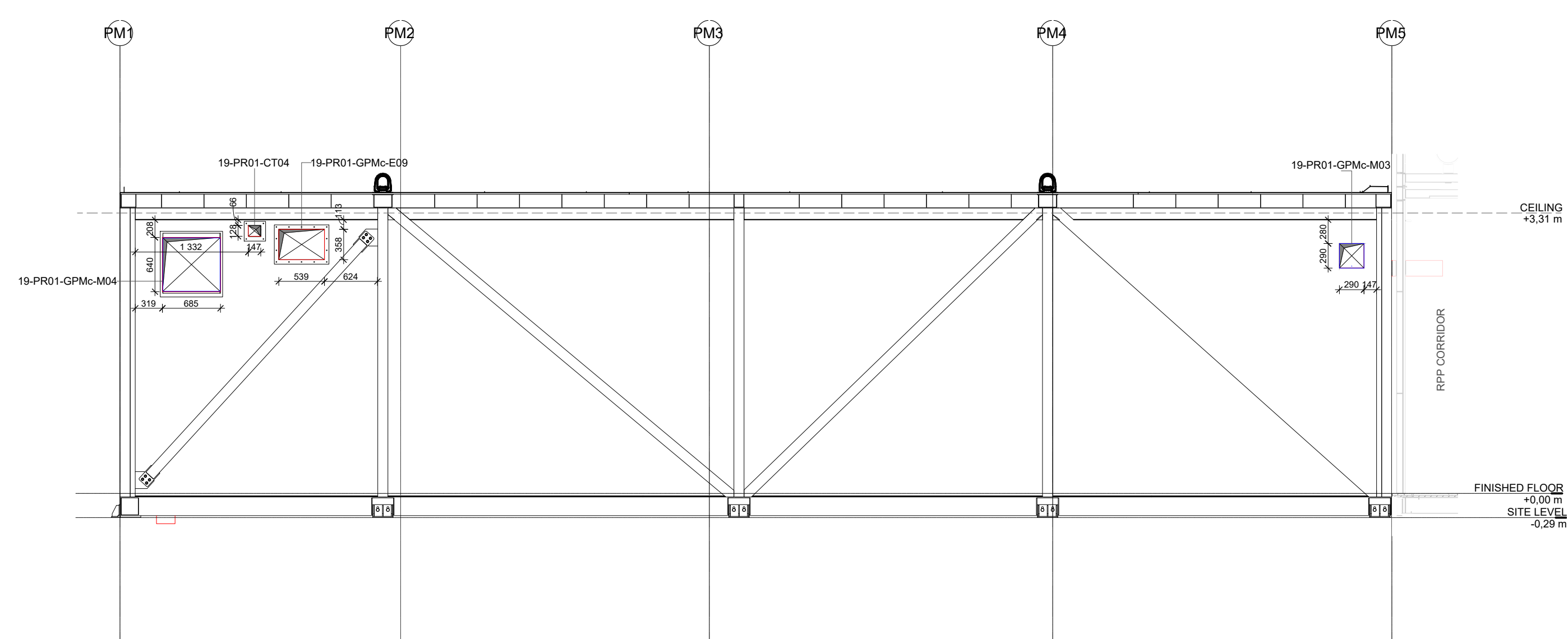
② PM-ELEVATION SOUTH 1 : 50
