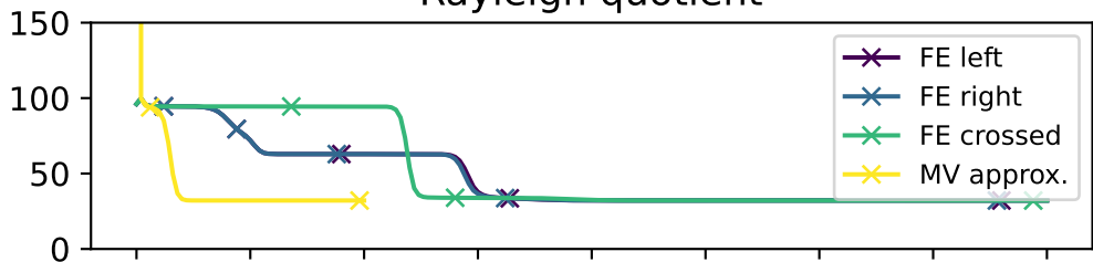
cosim
