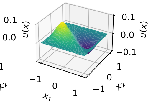
computed eigenfunction
