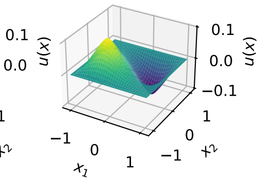
computed eigenfunction
