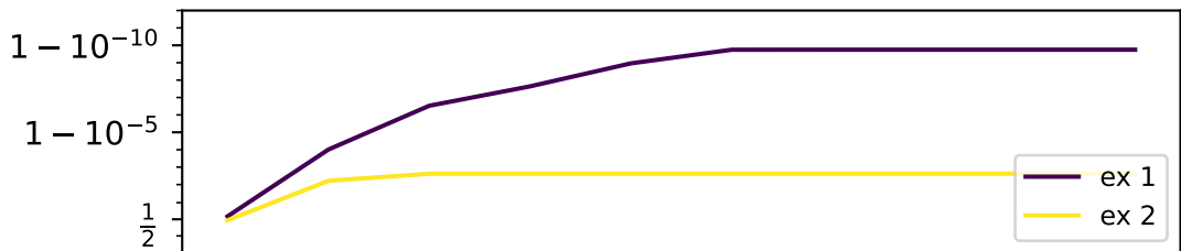
duality gap
