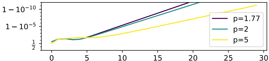
duality gap
