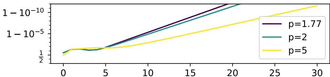
duality gap
