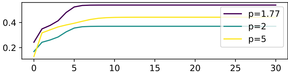
cosim
