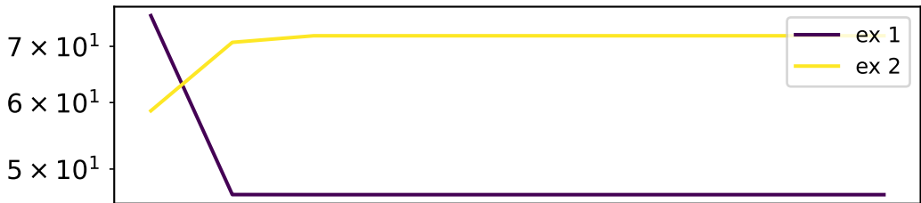
cosim
