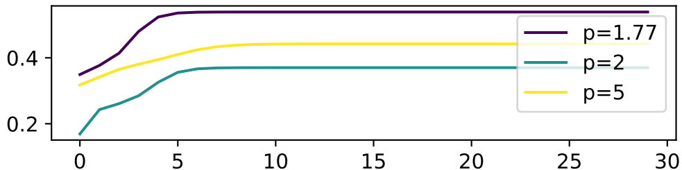
cosim
