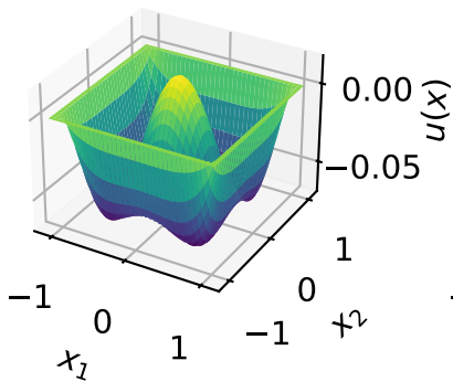
initial guess
