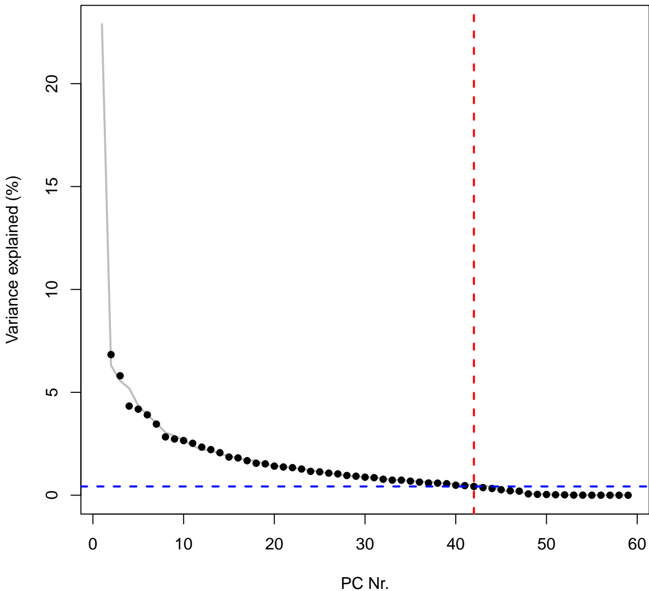
Scree Plot Cutoff: 0.5 % (blue line) at PC 42 (red line)
