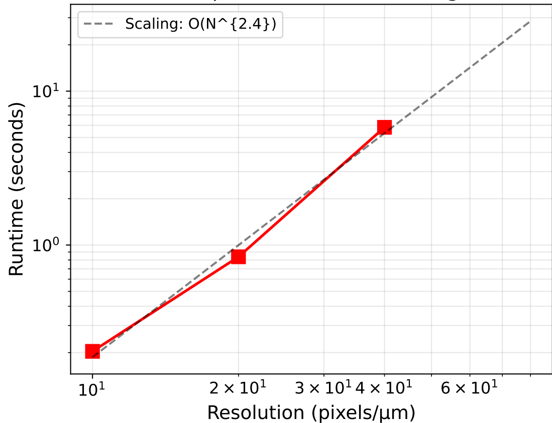
Computational Cost Scaling
