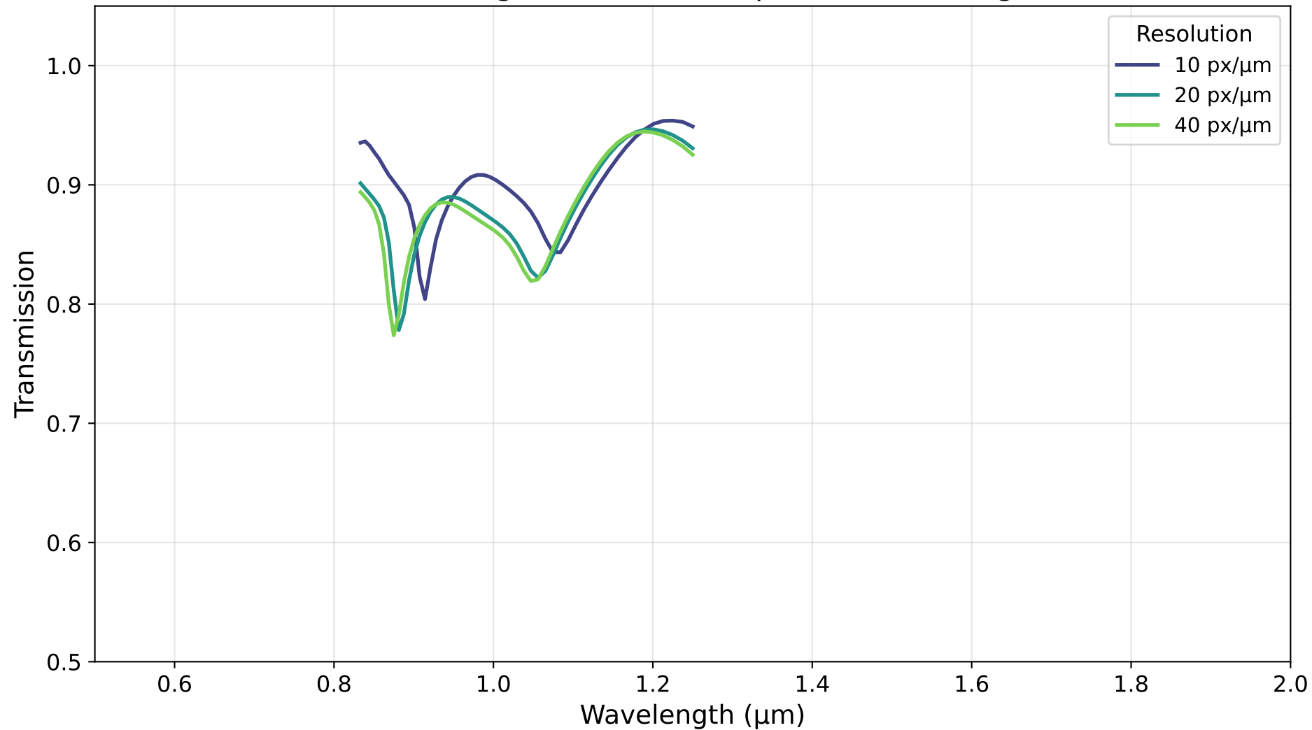
Mie Scattering: Transmission Spectrum Convergence
