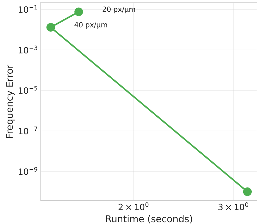
(a) Photonic Cavity: Cost vs Accuracy
