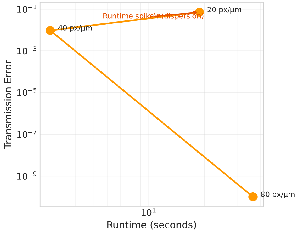
(b) Waveguide: Cost vs Accuracy
