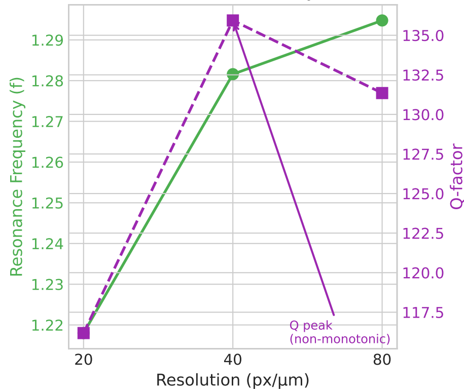
(b) Photonic Cavity
