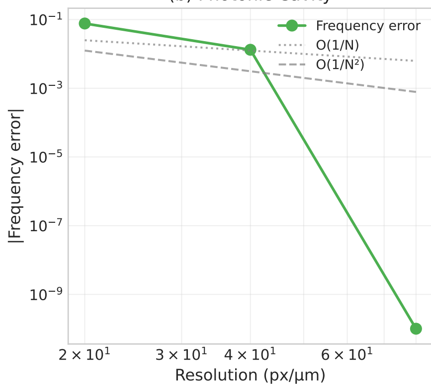
(b) Photonic Cavity
