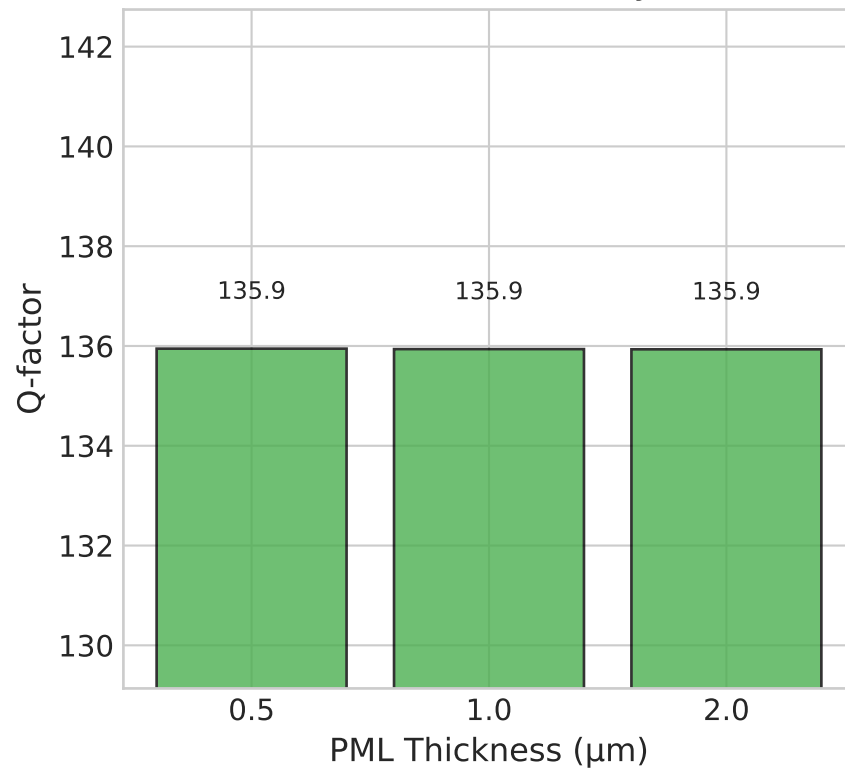
(b) Photonic Cavity
