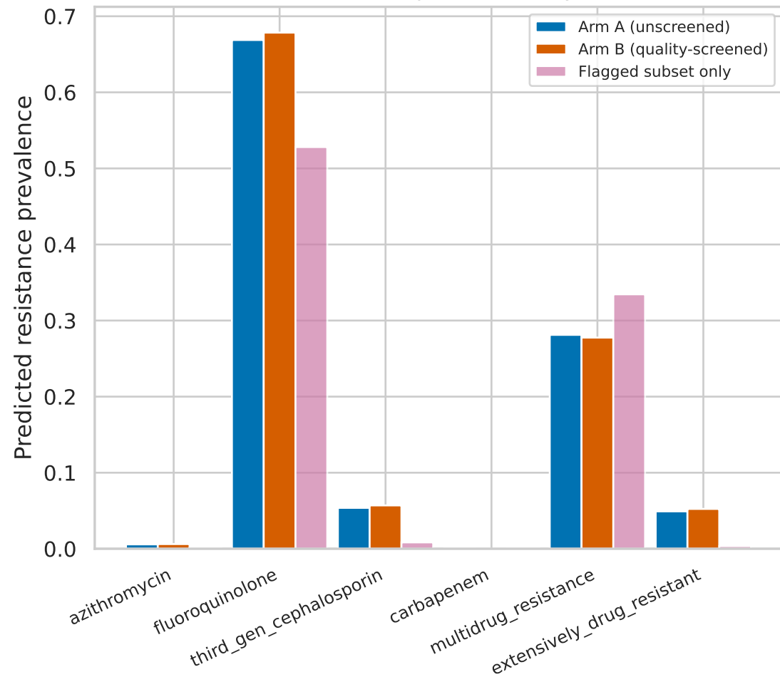
(a) Resistance prevalence by arm
