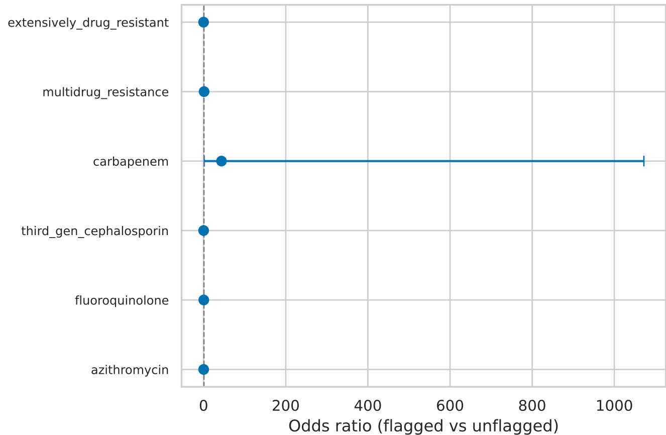
(b) Odds ratios, 95% CI
