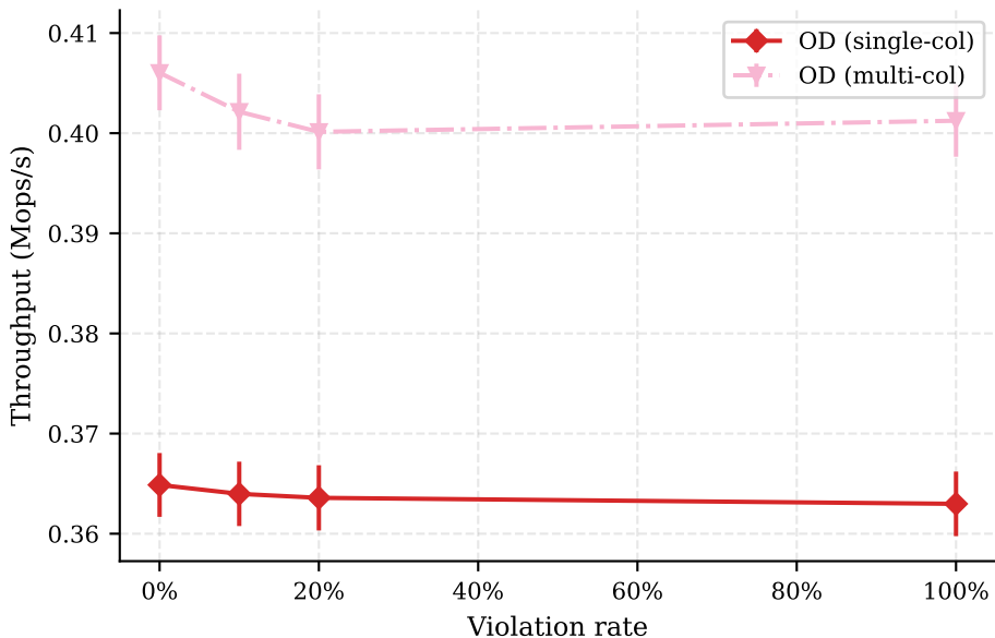
Delete - violation rate impact
