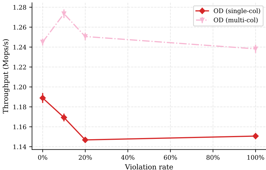
Lookup - violation rate impact
