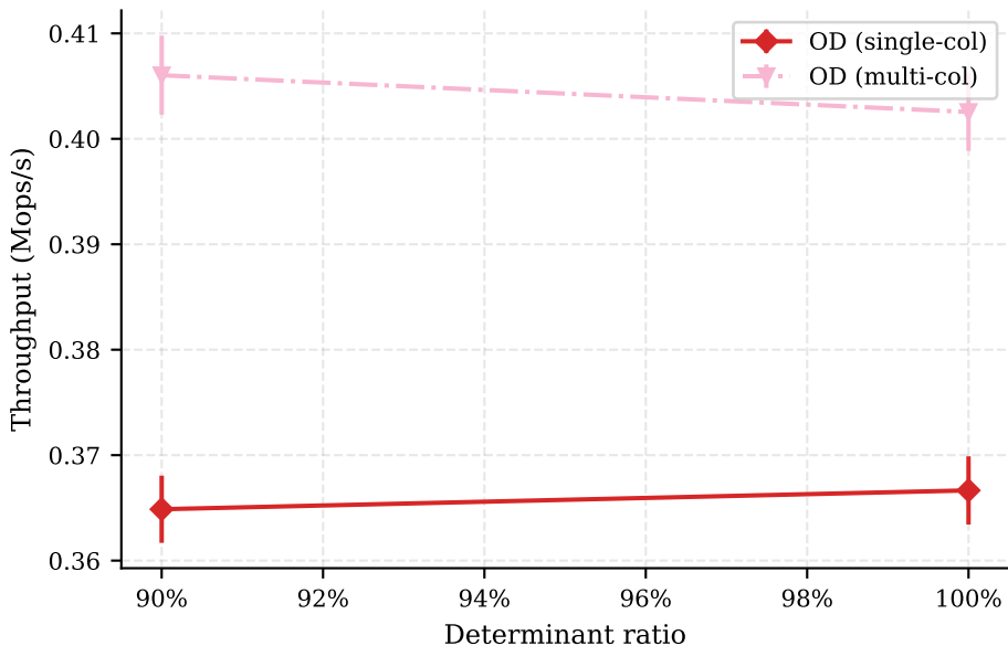
Delete - determinant ratio impact
