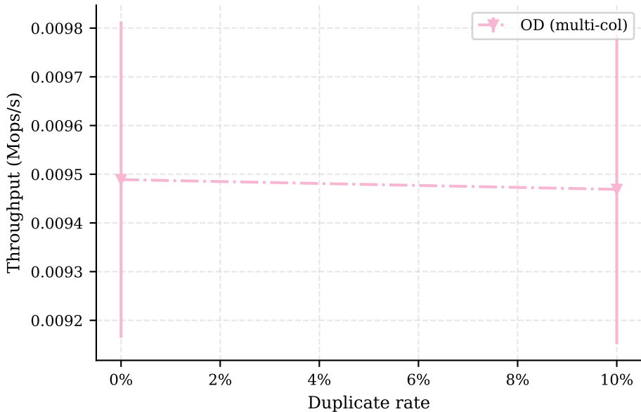
T4 - Throughput vs. duplicate rate
