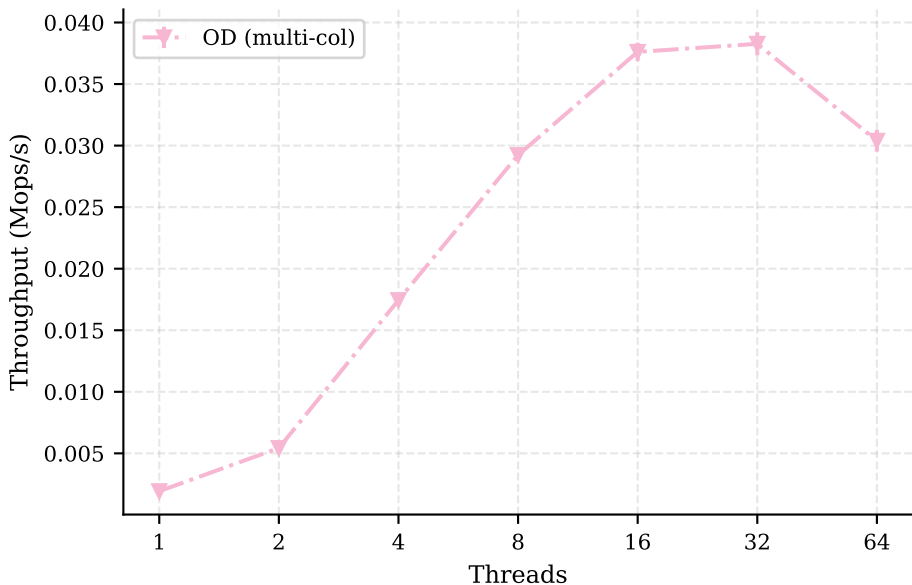
T5 - Throughput vs. thread count
