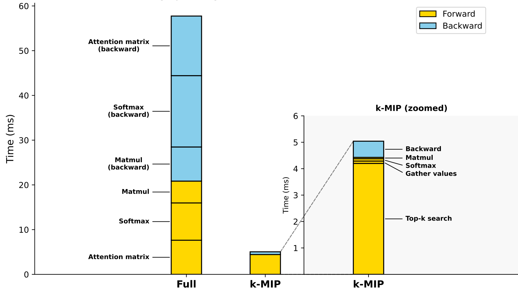
Per-stage profiling: Full vs k-MIP Attention ( N = 10^{4.5} )
