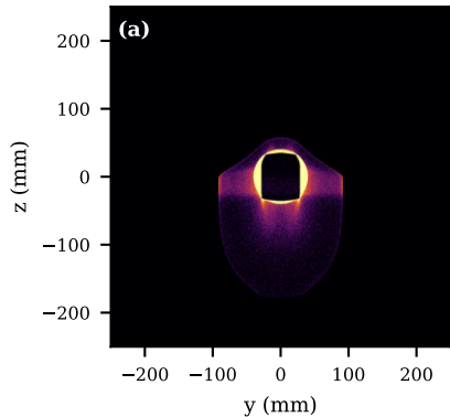
Monoenergetic 14.7 MeV
