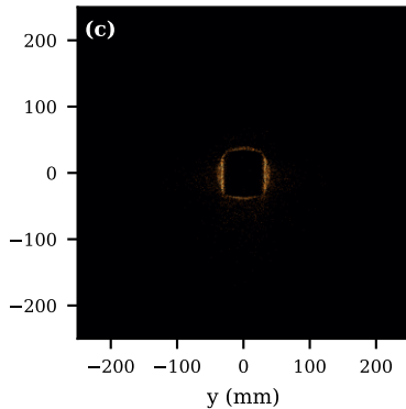
TNSA exponential T = 3 \text{ MeV}, E_{\text{cut}} = 40 \text{ MeV}
