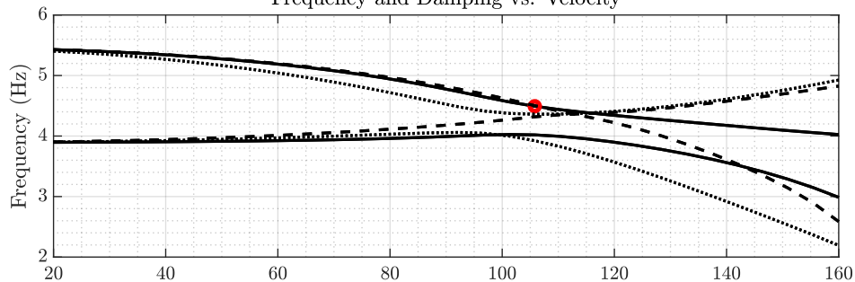
Frequency and Damping vs. Velocity
