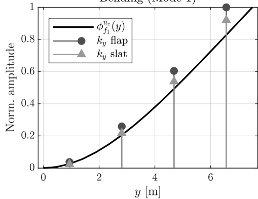
Bending (Mode 1)
