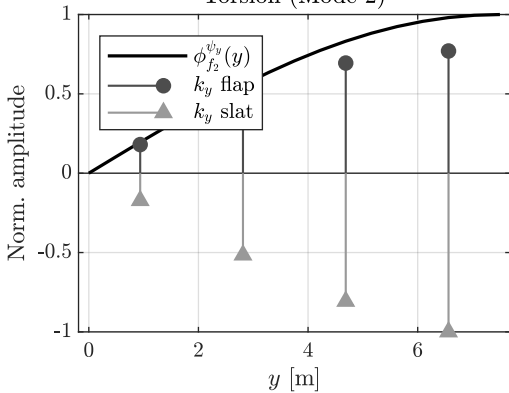
Torsion (Mode 2)
