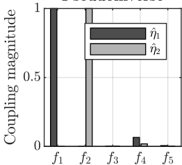
Pseudoinverse
