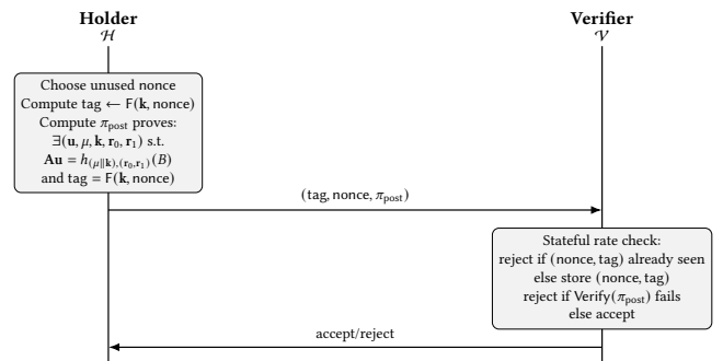
Figure 2: Showing (ARC presentation). Using an unused nonce \leq \text{presentation}_{\text{limit}} , the holder computes a deterministic tag from (\mathbf{k}, \text{nonce}) (rate limiting) and pseudorandom across unused nonces (unlinkability).
