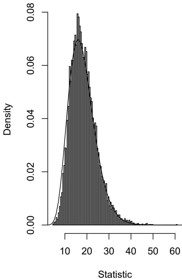
Marginal guessing distribution
