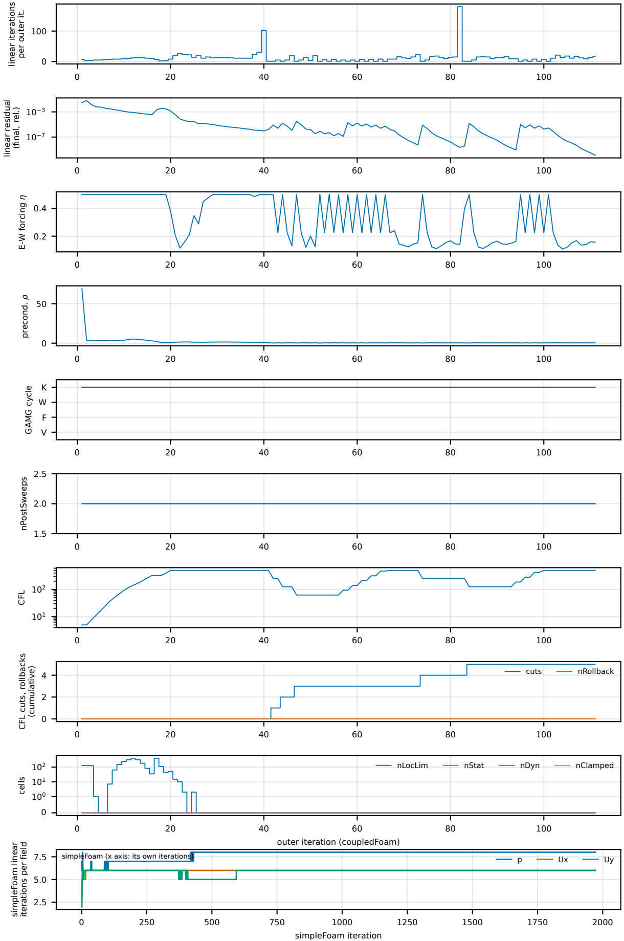
T0 cavity, Re 1000, 1 rank: linear solver and controls per outer iteration (dotted: GAMG autoTune events)
