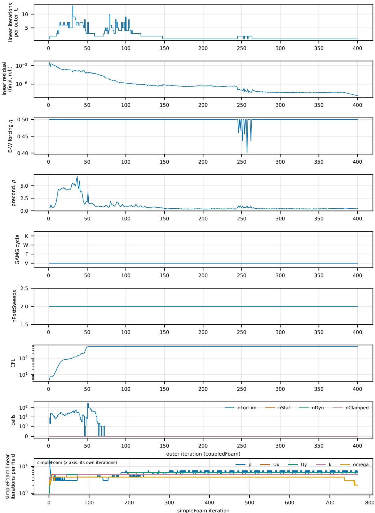
T1 pitzDaily, 4 ranks: linear solver and controls per outer iteration (dotted: GAMG autoTune events)
