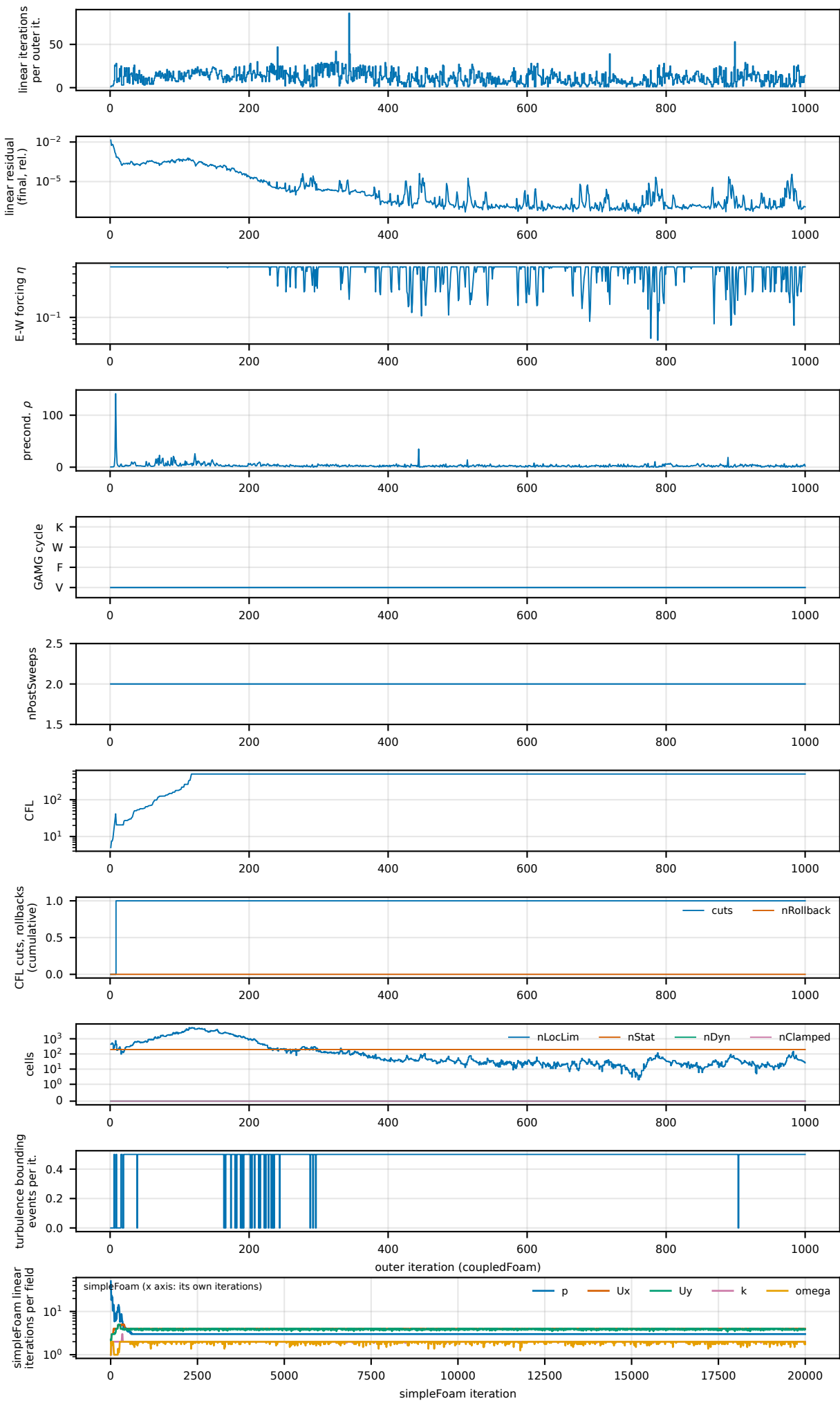
T2 backward-facing step, 1 rank: linear solver and controls per outer iteration (dotted: GAMG autoTune events)
