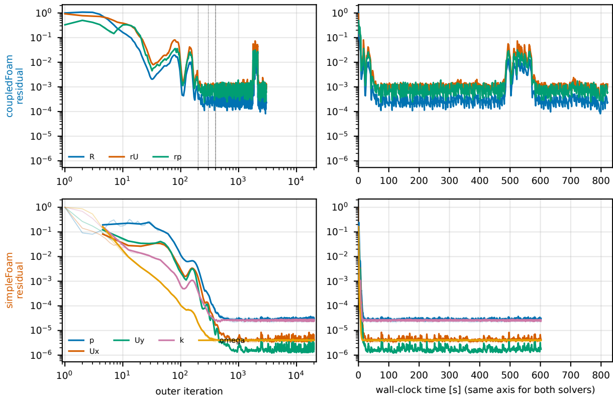
T3 airFoil2D, GEKO: residuals (coupledFoam: combined R , momentum r_U , continuity r_p ; simpleFoam: initial residuals; long runs: band = per-bin min/max, line = bin mean). Same y range; normalisations differ.
