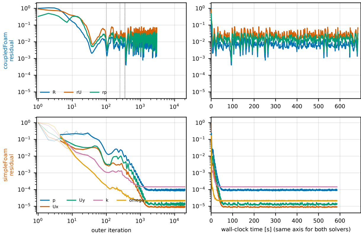
T3 airFoil2D, SST: residuals (coupledFoam: combined R , momentum r_U , continuity r_p ; simpleFoam: initial residuals; long runs: band = per-bin min/max, line = bin mean). Same y range; normalisations differ.
