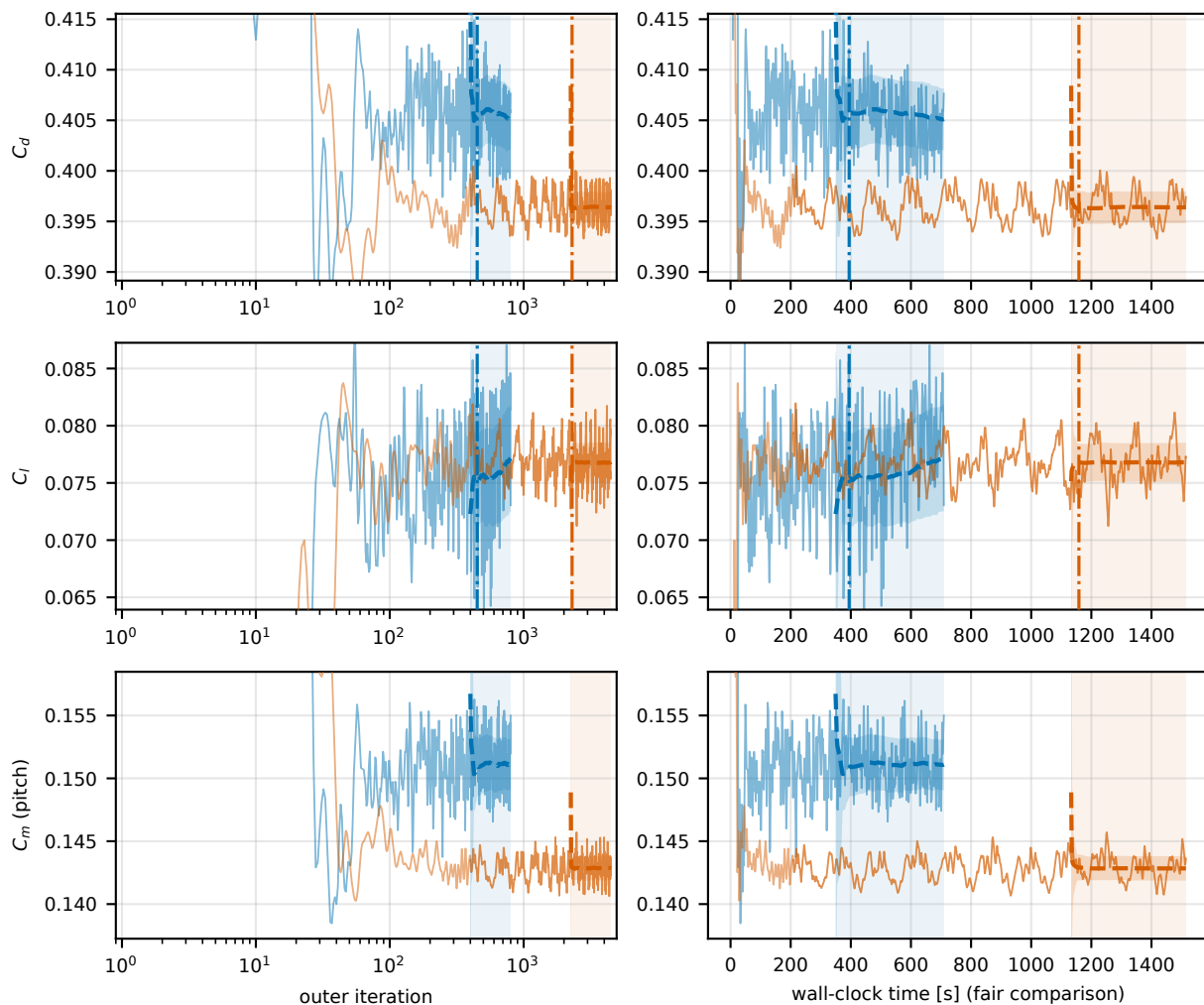
T4a motorBike, 354k cells, 10 ranks: monitored quantities (dash-dot: iterations to stationary window, D-042; shading: final averaging window)
