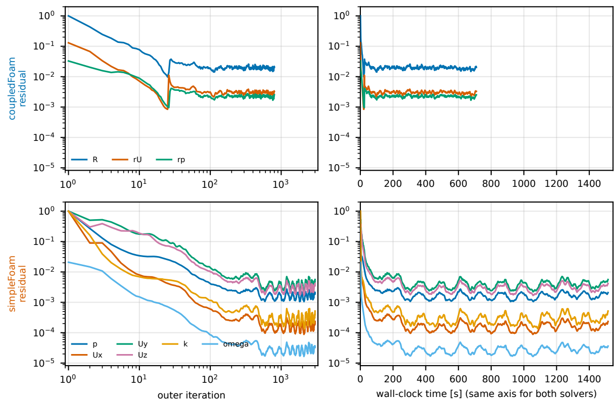
T4a motorBike, 354k cells, 10 ranks: residuals (coupledFoam: combined R , momentum r_U , continuity r_p ; simpleFoam: initial residuals; long runs: band = per-bin min/max, line = bin mean). Same y range; normalisations differ.
