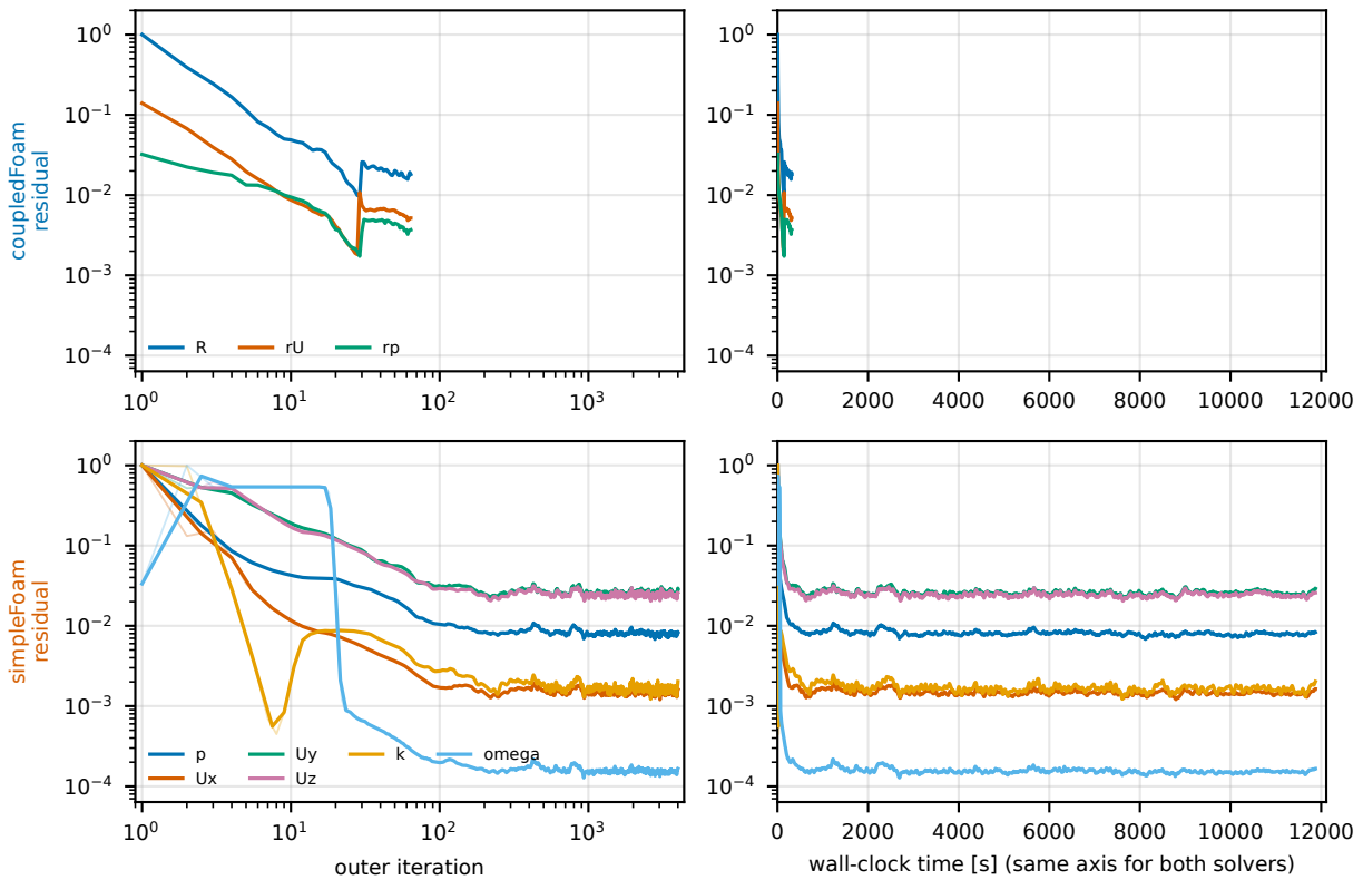
T4b motorBike, 1.70M cells, 10 ranks: residuals (coupledFoam: combined R , momentum r_U , continuity r_p ; simpleFoam: initial residuals; long runs: band = per-bin min/max, line = bin mean). Same y range; normalisations differ.
