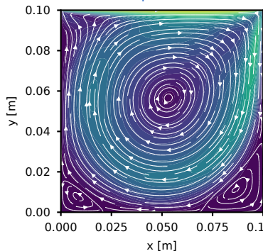
coupledFoam
