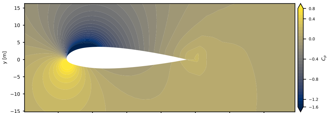
simpleFoam
