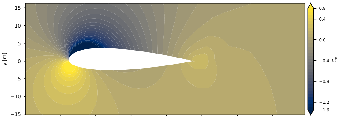
coupledFoam
