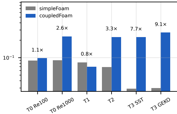
wall time per outer iteration [s]
