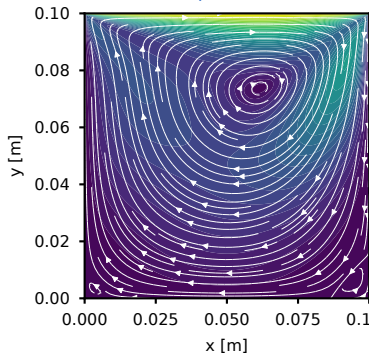
coupledFoam
