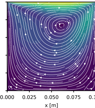
simpleFoam
