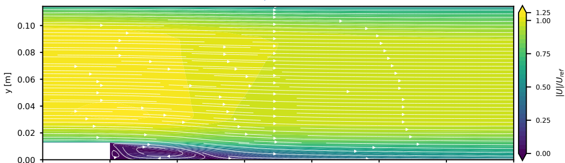
simpleFoam
