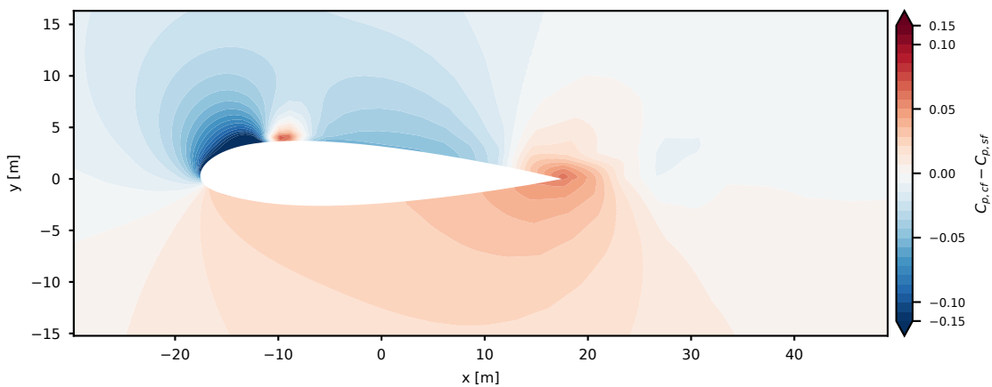
delta: RMS 3.19e-03, max 1.83e-01
